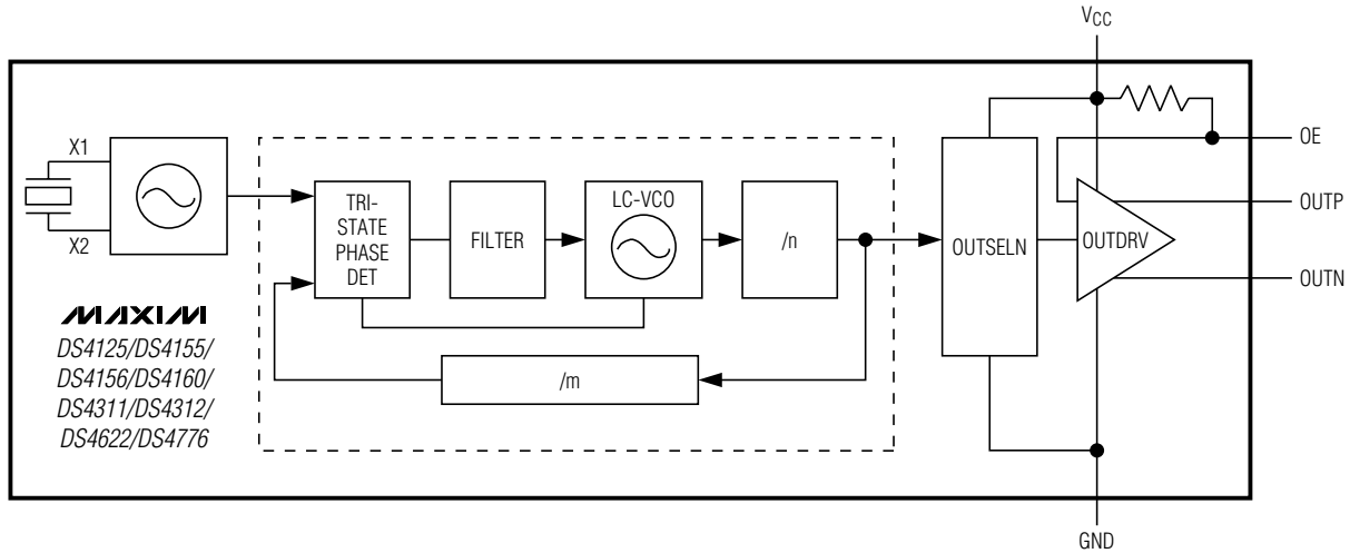
Figure 1. Functional Diagram
