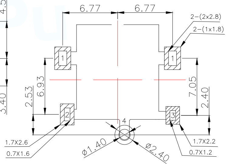
PCB.WELDING DRAWING (TOLERANCE:±0.05)
