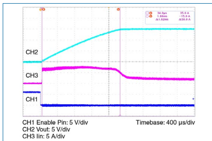
Figure 4 — Inrush current at nominal line 15% load; 5 A/div, Max load capacitance
