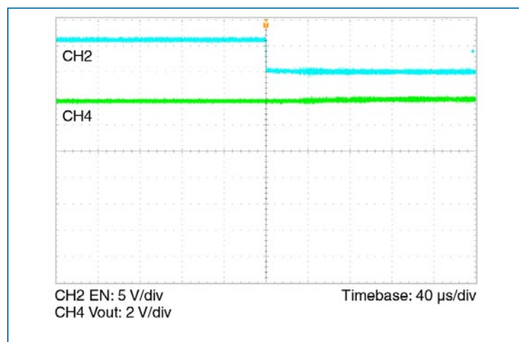
Figure 18 — Three module parallel array test. V_{out} change with two modules operating and a third module enabled. Nominal V_{in} , I_{out} = 96 A
