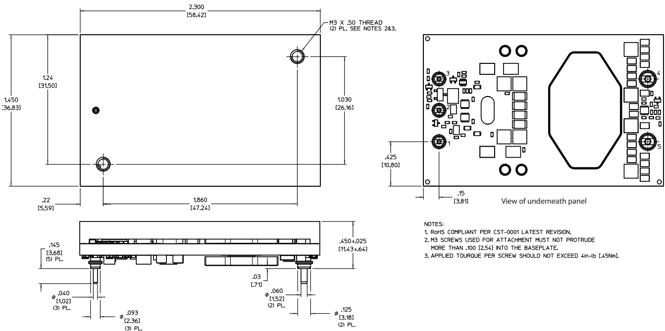
Figure 32 — IBC outline drawing - baseplate option
