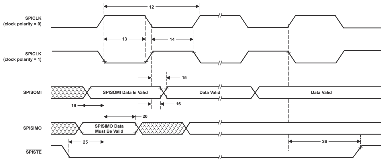
Figure 7-82. High-Speed SPI Slave Mode External Timing (Clock Phase = 1)
