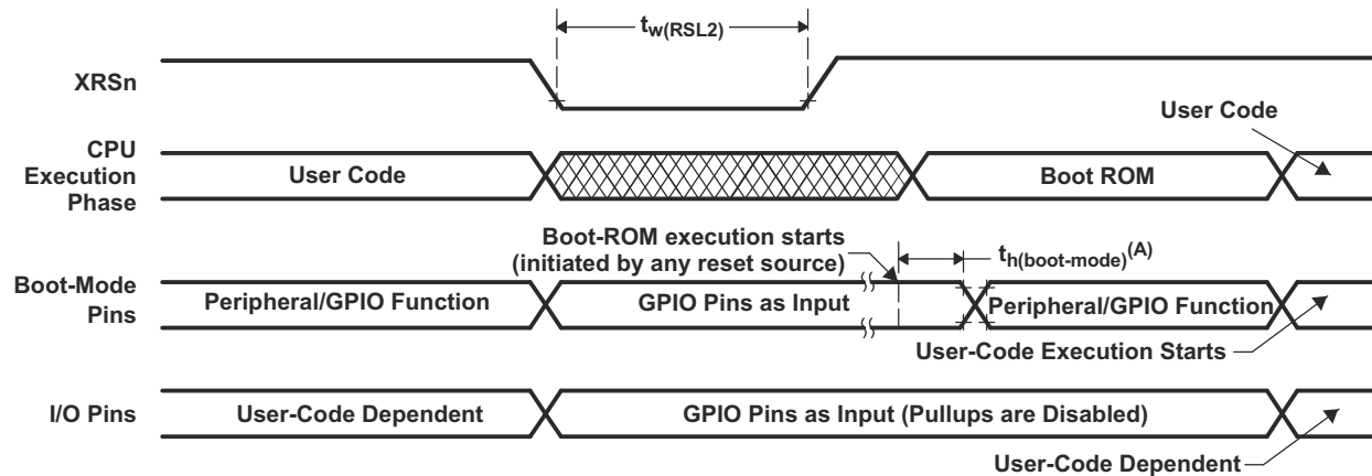
Figure 7-9. Warm Reset
