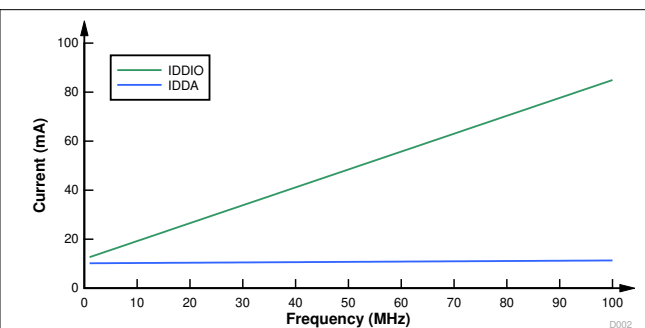
Figure 7-3. Current Versus Frequency — Internal VREG
