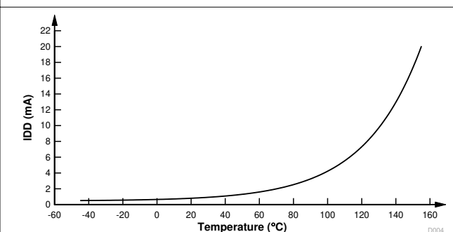
Figure 7-5. Halt Current Versus Temperature (°C)
