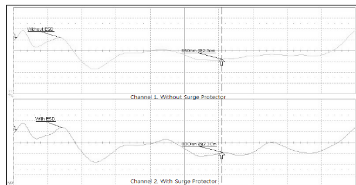
Figure 6. TDR Test Result
