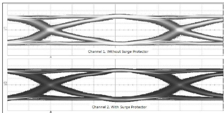
Figure 5. Eye Diagram
