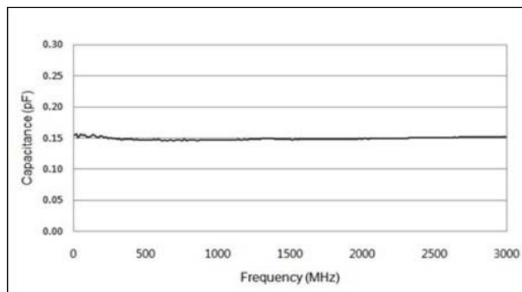
Figure 2. Capacitance
