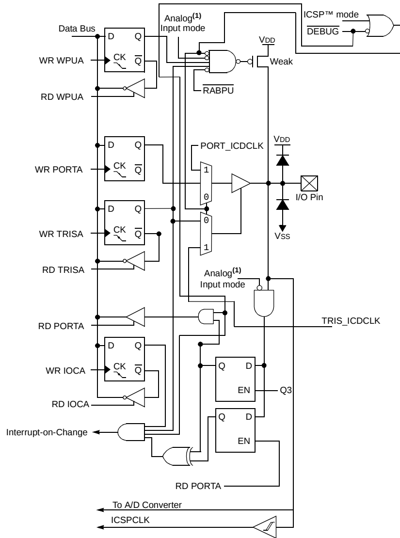
FIGURE 6-2: BLOCK DIAGRAM OF RA1
