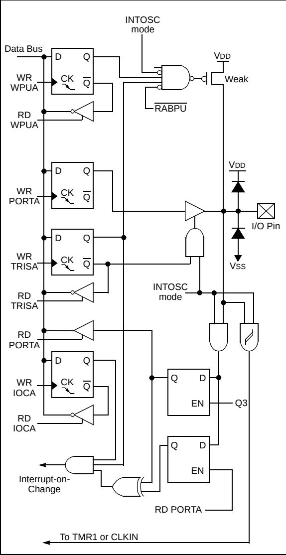
FIGURE 6-6: BLOCK DIAGRAM OF RA5
