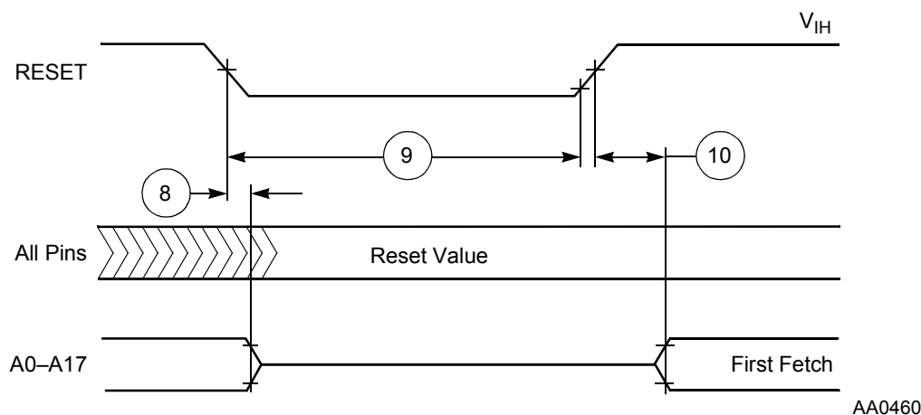
Figure 2-2 Reset Timing
