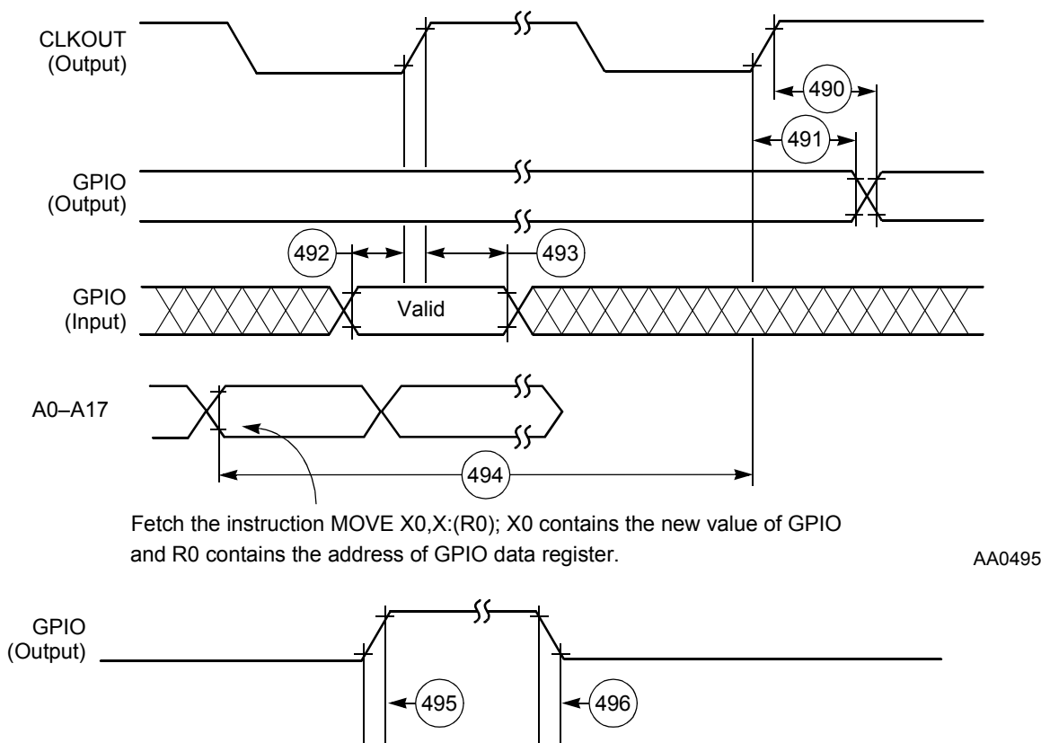
Figure 2-48 GPIO Timing
