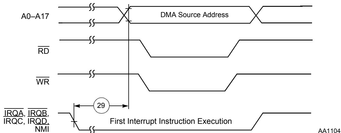
Figure 2-10 External Memory Access (DMA Source) Timing
