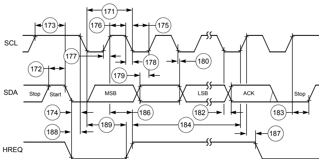
Figure 2-39 I 2 C Timing
