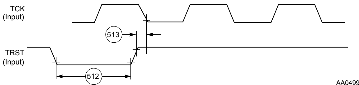
Figure 2-52 TRST Timing Diagram
