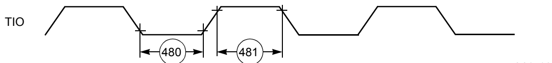
Figure 2-45 TIO Timer Event Input Restrictions
