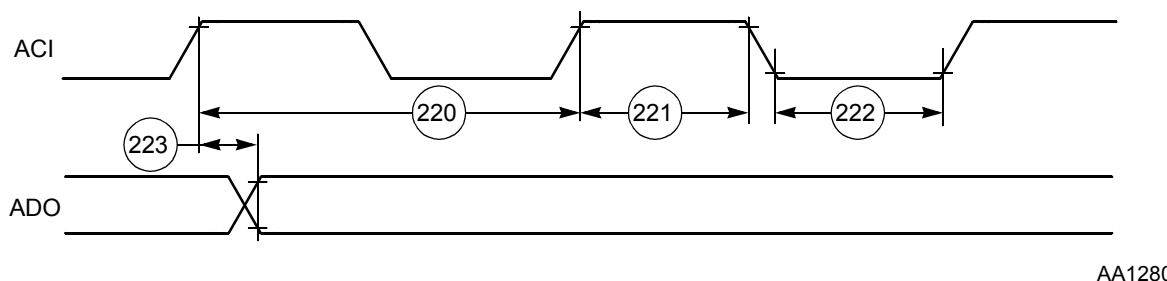
Figure 2-44 Digital Audio Transmitter Timing
