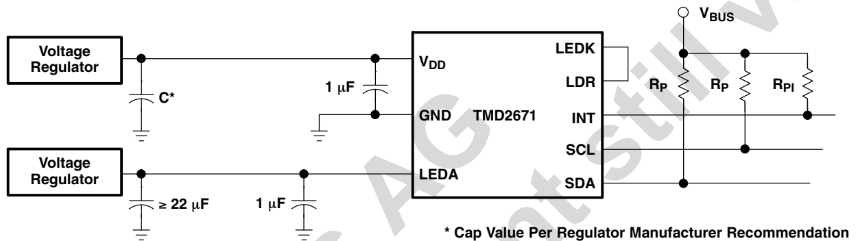
Figure 12. Proximity Sensing Using Separate Power Supplies
