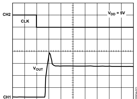
CH1 1V, CH2 5V, TIME BASE = 5 \mu s/DIV
