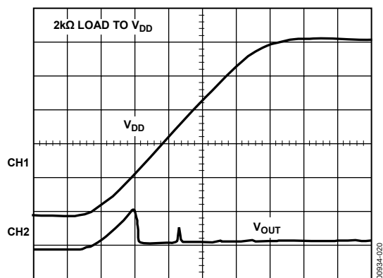
CH1 1V, CH2 1V, TIME BASE = 20 \mu s/DIV
