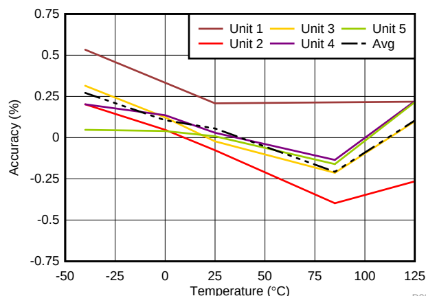
V_{ITN} Accuracy vs Temperature
