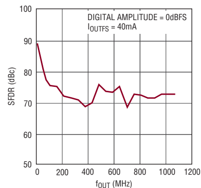
SFDR vs f_{OUT} , f_{DAC} = 2.7\text{Gpsps}
