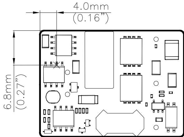
Figure 20: Temperature measurement location The allowed maximum hot spot temperature is defined at 113 °C.
