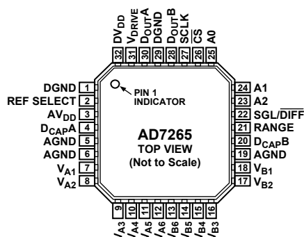
Figure 2. 32-Lead CP-32-2
