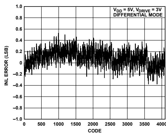
Figure 9. Typical INL
