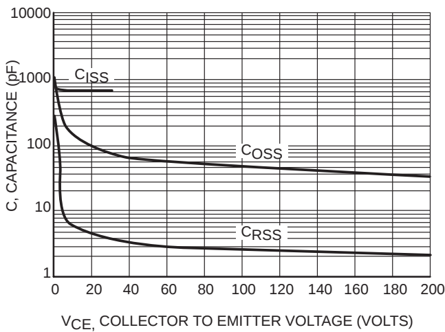
Figure 5. Capacitance Variation
