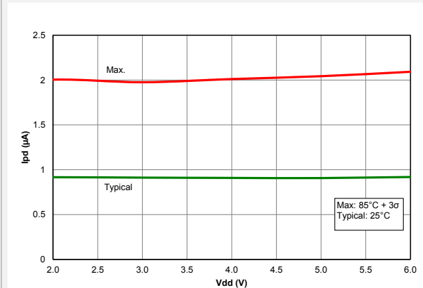
Figure 41-62. I_{PD} , Watchdog Timer, PIC18F67K40 only
