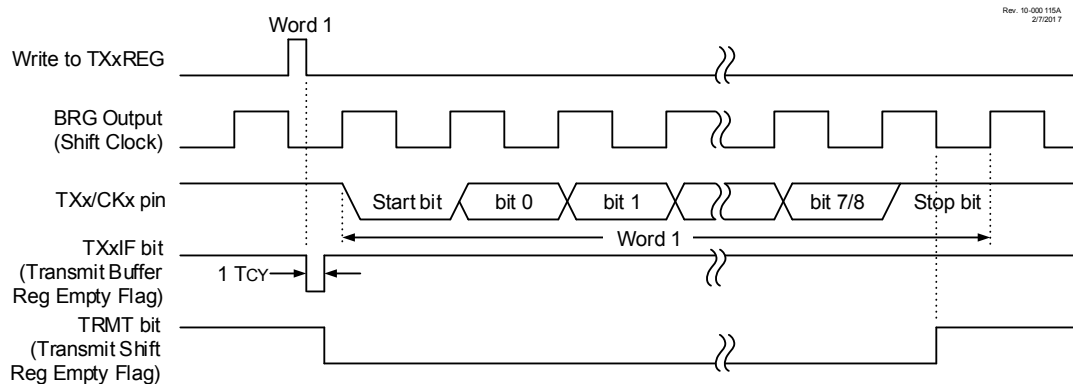
Figure 29-3. Asynchronous Transmission
