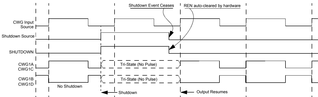
Figure 25-18. SHUTDOWN FUNCTIONALITY, AUTO-RESTART ENABLED (REN = 1, LSAC = 01, LSBD = 01)
