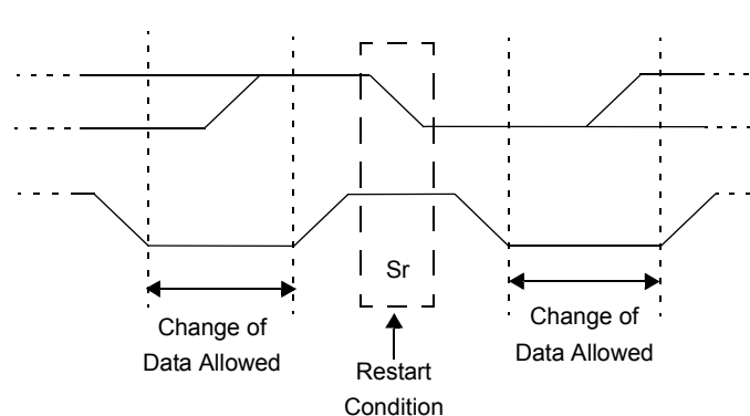
Figure 28-13. I 2 C Restart Condition
