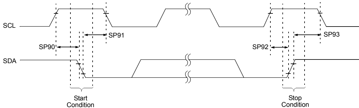
Figure 40-20. I 2 C Bus Start/Stop Bits Timing
