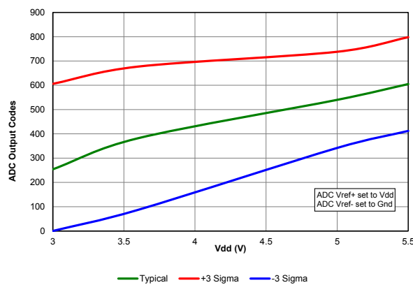
Figure 41-85. Temperature Indicator, Initial Offset, High Range, Temp = 20°C, PIC18F67K40 only
