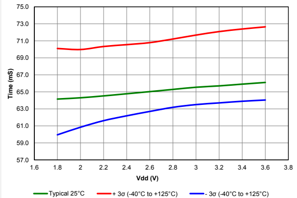
Figure 41-84. Power-up Timer Period, PIC18LF67K40 only
