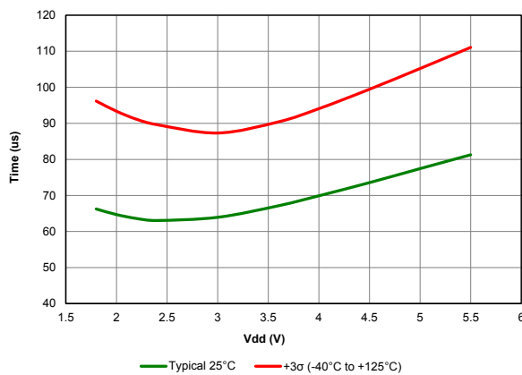
Figure 41-103. Wake From Sleep, VREGPM = 1, HFINTOSC = 16MHz
