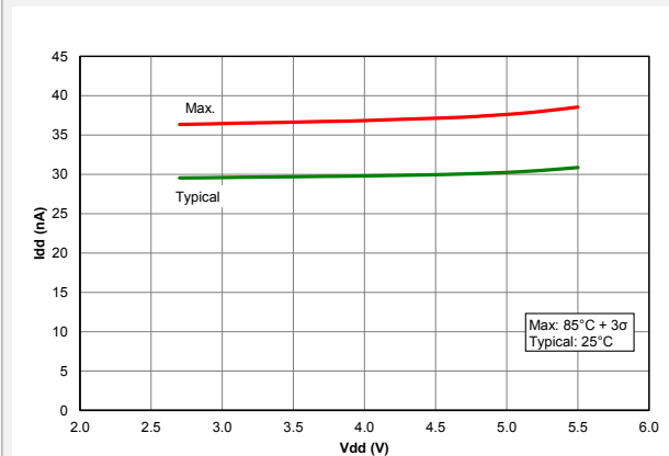
Figure 41-64. I_{DD} , Fixed Voltage Reference (FVR), PIC18F67K40 only
