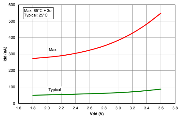
Figure 41-71. I_{PD} Base, Low-power Sleep Mode, PIC18LF67K40 only
