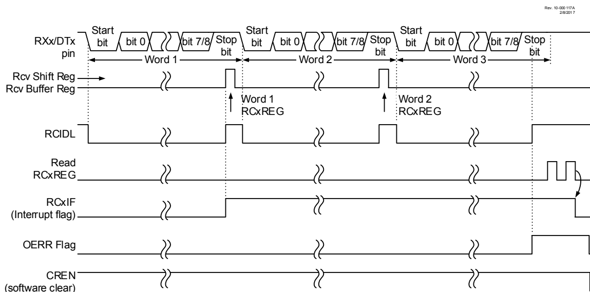
Figure 29-5. Asynchronous Reception
