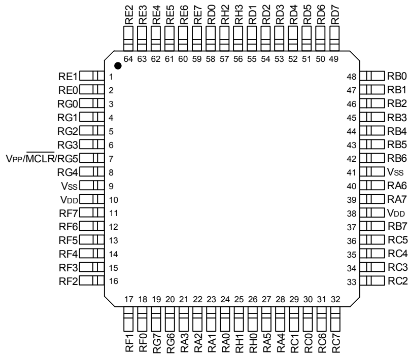
Figure 1. 64-pin TQFP
