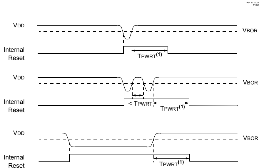
Figure 18-2. Brown-out Situations
