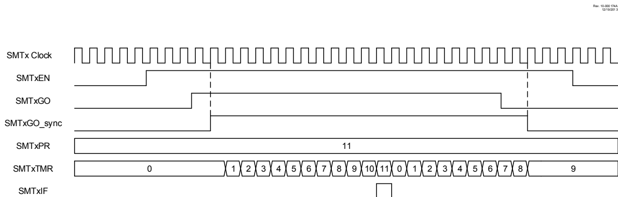
Figure 26-2. Timer Mode Timing Diagram
