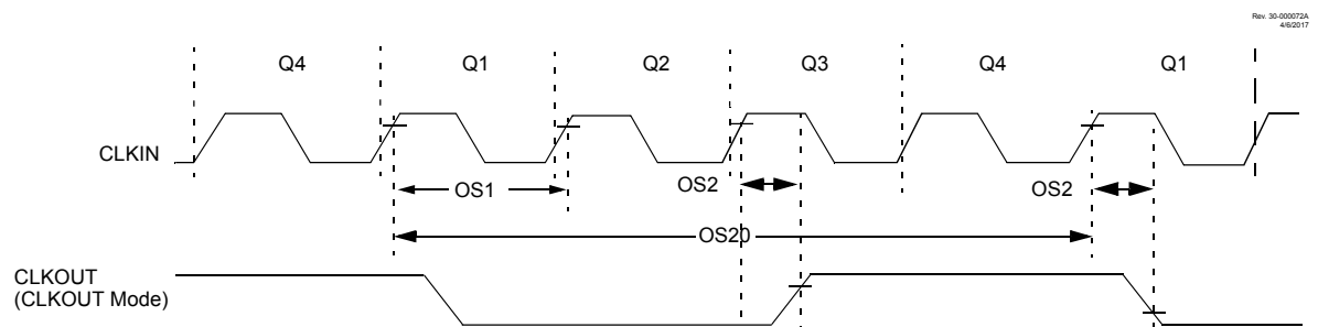
Figure 40-5. Clock Timing
