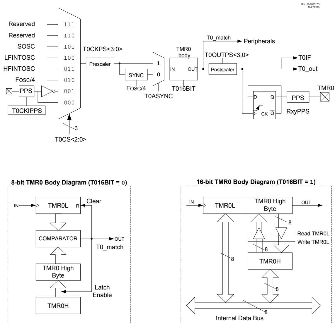
Figure 19-1. Block Diagram of Timer0
