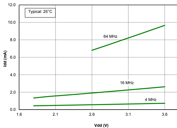
Figure 41-53. I_{DD} , HFINTOSC, Typical, PIC18LF67K40 only
