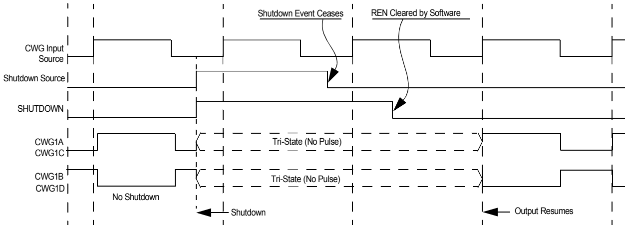
Figure 25-17. SHUTDOWN FUNCTIONALITY, AUTO-RESTART DISABLED (REN = 0, LSAC = 01, LSBD = 01)
