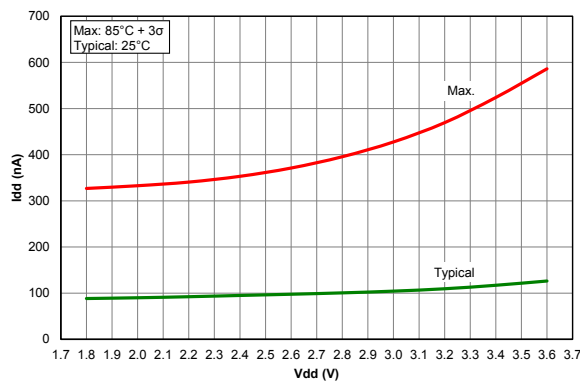
Figure 41-69. I_{PD} , Comparator, PIC18LF67K40 only
