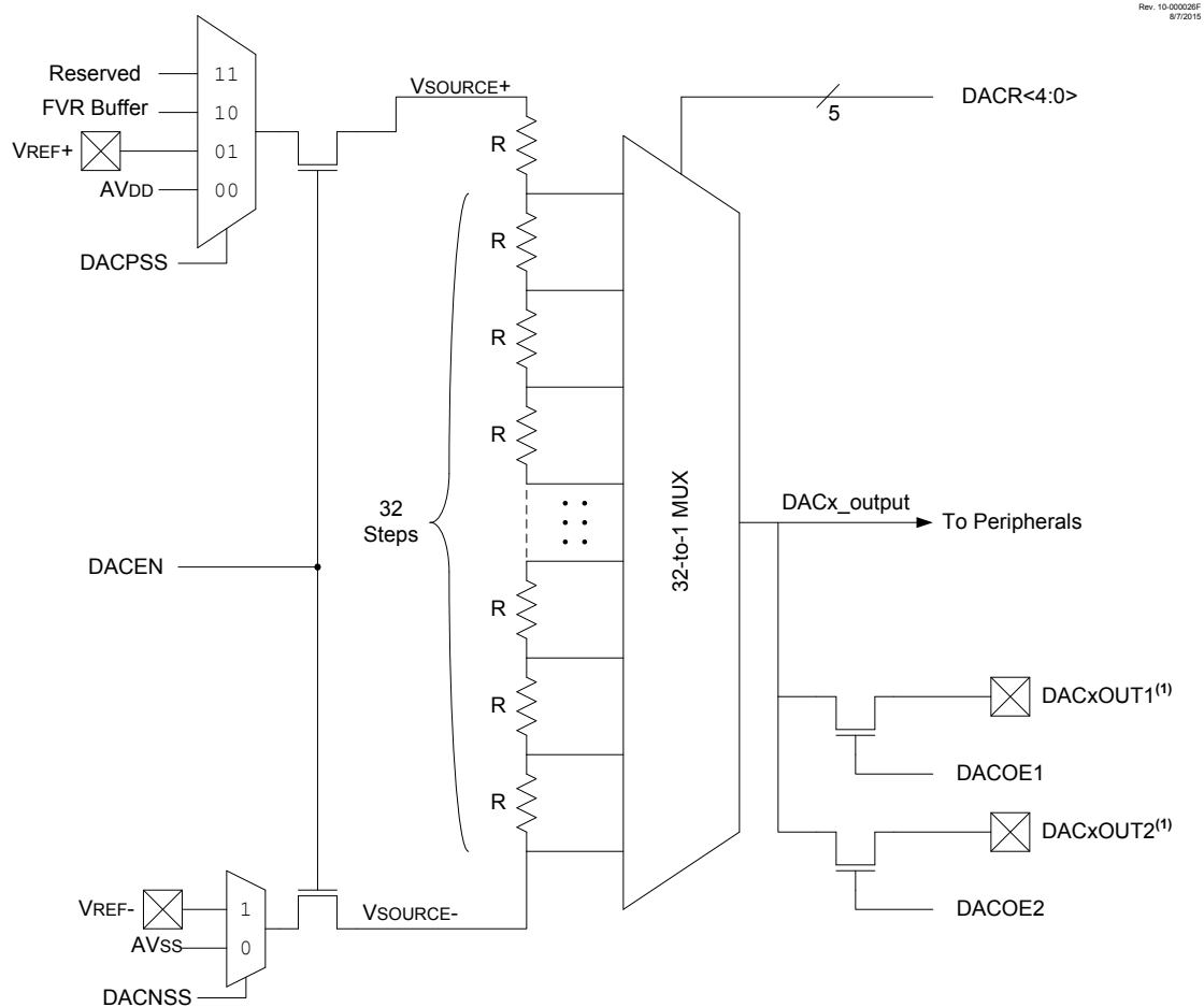
Figure 32-1. Digital-to-Analog Converter Block Diagram
