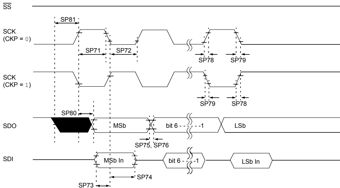
Figure 40-16. SPI Master Mode Timing (CKE = 0, SMP = 0)
