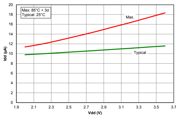
Figure 41-67. I_{PD} , Low-power Brown-out Reset, LPBOR = 0, PIC18LF67K40 only
