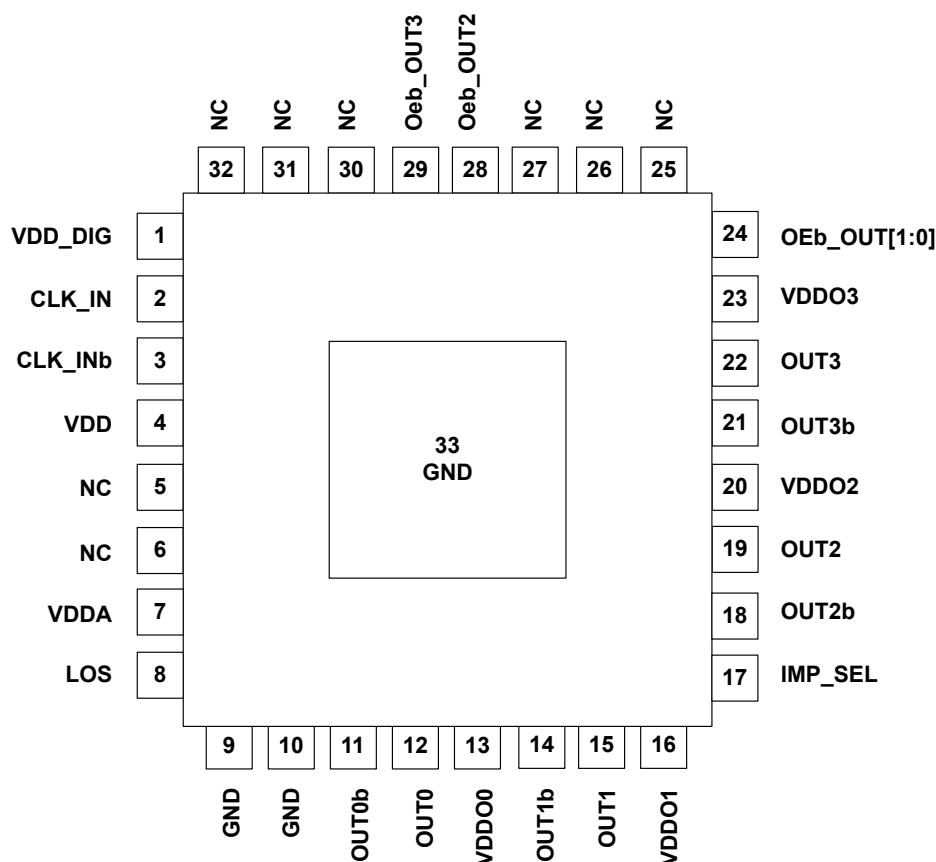
Figure 6.3. Si53254A-D01AM 32-QFN
