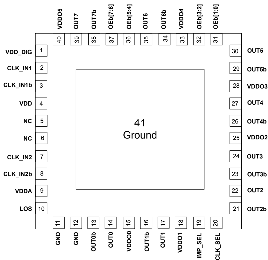
Figure 6.2. Si53258A-D02-AM 40-QFN
