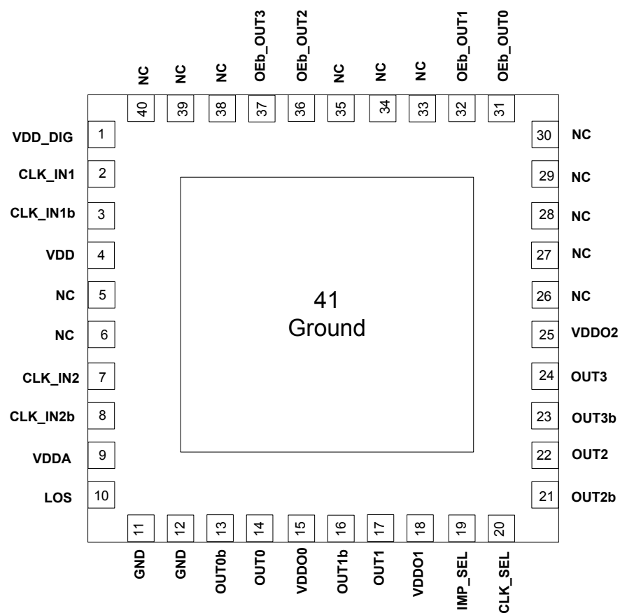
Figure 6.4. Si53254A-D02AM 40-QFN
