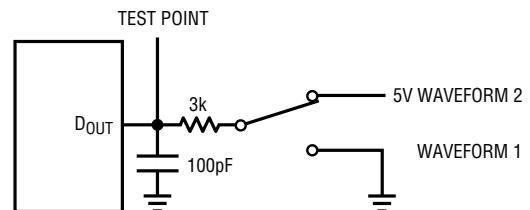
Load Circuit for t_{\text{dis}} and t_{\text{en}}
