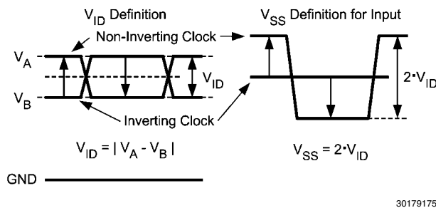
FIGURE 11. Two Different Definitions for Differential Input Signals
