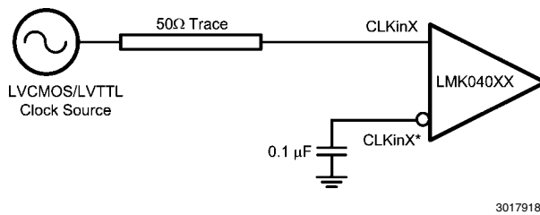
FIGURE 27. DC Coupled LVCMOS/LVTTL Reference Clock
