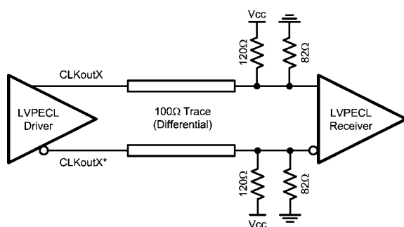
FIGURE 30. Differential LVPECL Operation, DC Coupling, Thevenin Equivalent
