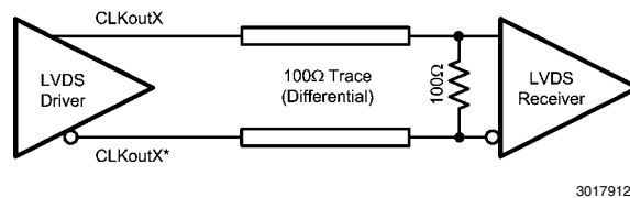
FIGURE 28. Differential LVDS Operation, DC Coupling, No Biasing of the Receiver
