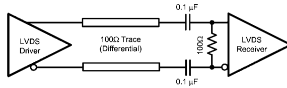
FIGURE 32. LVDS Termination for a Self-Biased Receiver
