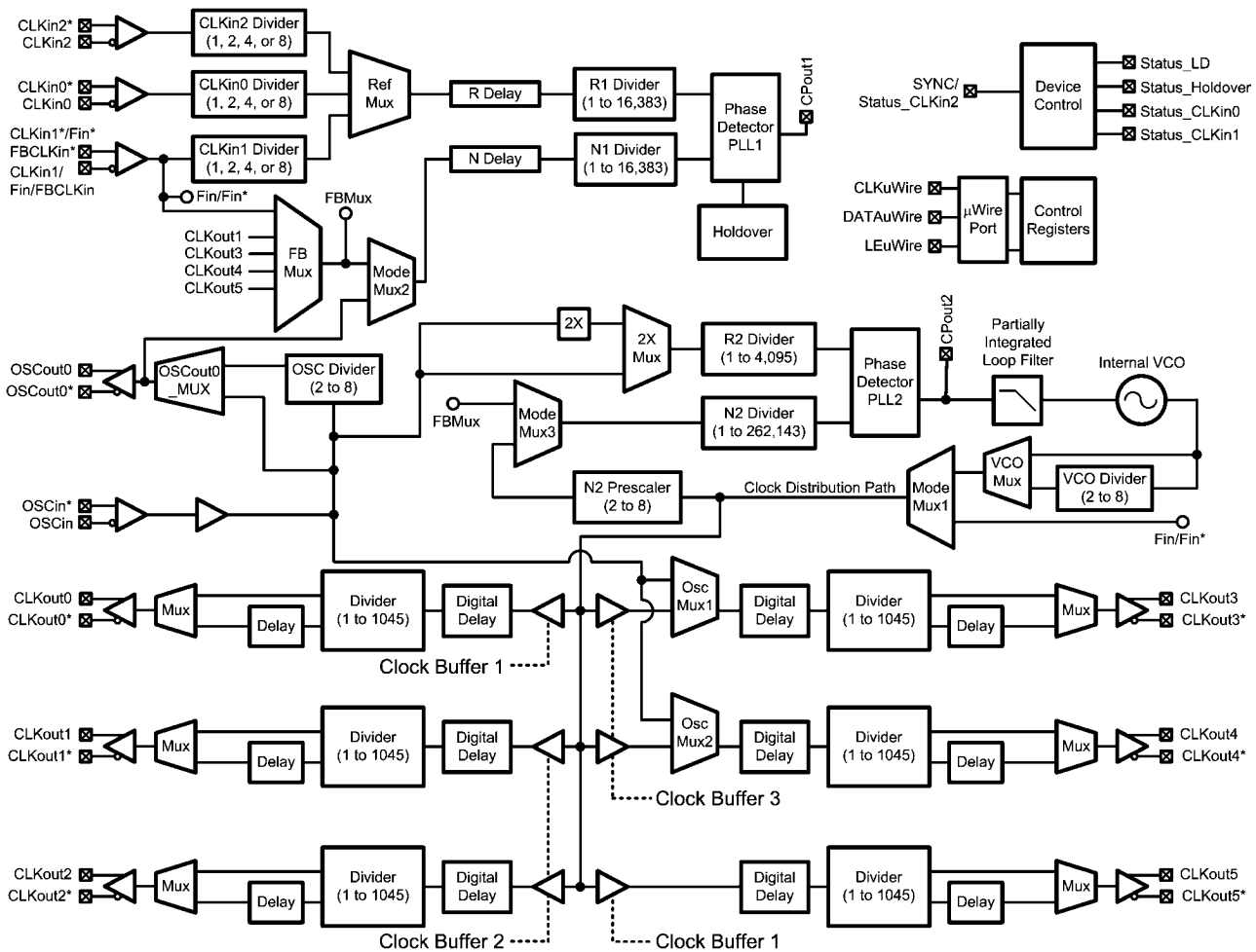
FIGURE 6. Detailed LMK04906 Block Diagram
