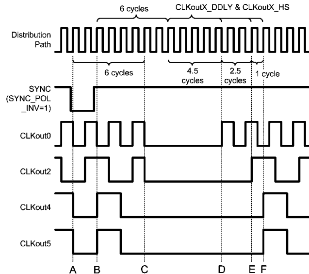
FIGURE 15. Clock Output synchronization using the SYNC pin (Active Low)
