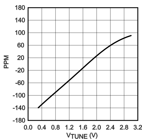
FIGURE 22. Example Tuning Curve, 20.48 MHz Crystal
