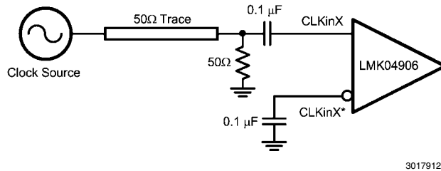
FIGURE 26. CLKInX/X* Single-ended Termination
