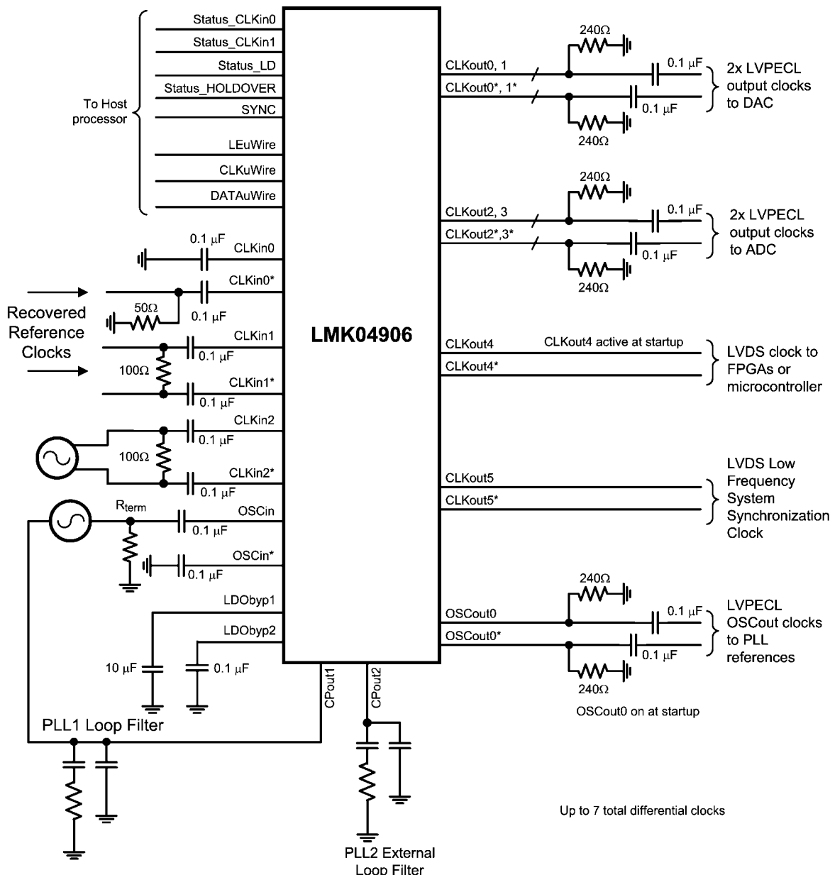
FIGURE 19. Example Application – System Schematic Except for Power
