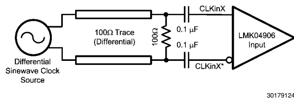
FIGURE 25. CLKInX/X* Termination for a Differential Sinewave Reference Clock Source
