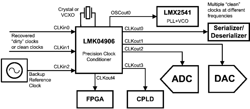
Simplified LMK04906 Block Diagram
