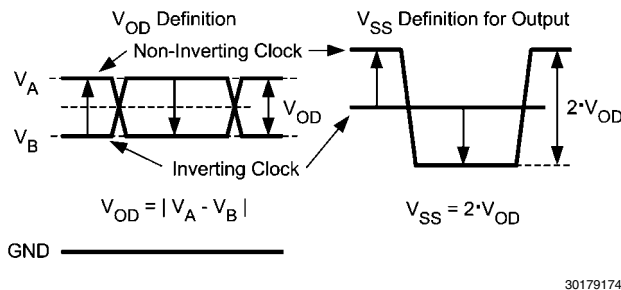
FIGURE 12. Two Different Definitions for Differential Output Signals
