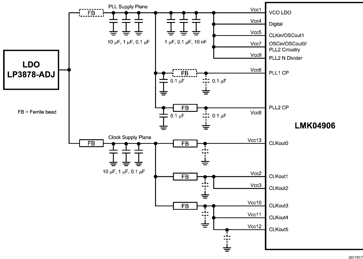
FIGURE 20. Example Application – Power System Schematic
