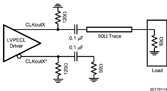
FIGURE 36. Single-Ended LVPECL Operation, AC Coupling
