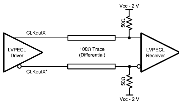
FIGURE 29. Differential LVPECL Operation, DC Coupling
