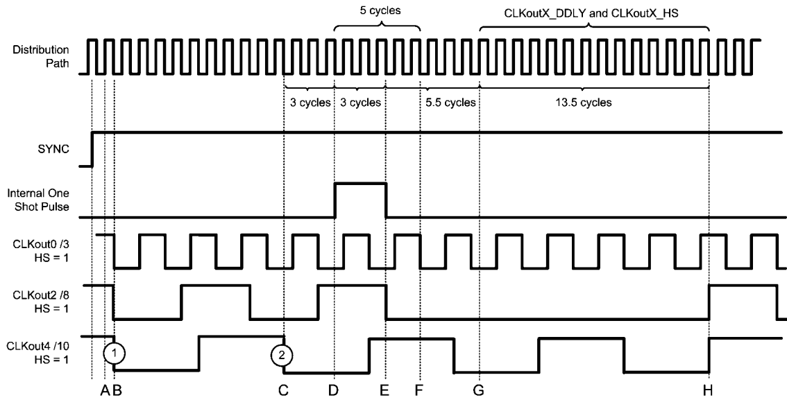
FIGURE 16. Absolute Dynamic Digital Delay Programming Example (SYNC_QUAL = 1, Qualify with clock output)
