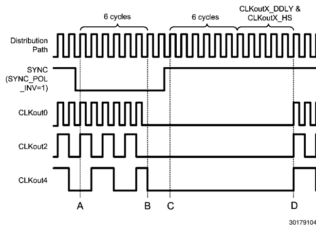
FIGURE 14. Clock Output synchronization using the SYNC pin (Active Low) CLKout0_DIV = 0 (valid only for external VCO mode) CLKout2_DIV = 2 CLKout4_DIV = 4 The digital delay for all clock outputs is 5 The digital delay half step for all clock outputs is 0 SYNC_QUAL = 0 (No qualification)
