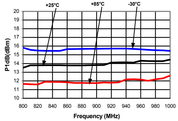
P1 dB vs. Frequency V_{dd} = 5 V
