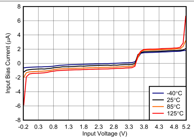
Figure 6-16. Bias Current vs. Input Voltage, 5 V
