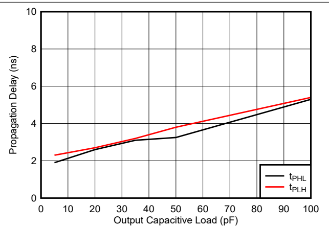
Figure 6-38. Propagation Delay vs. Load Capacitance, 5 V
