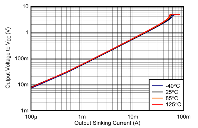
Figure 6-22. Output Voltage vs. Output Sinking Current, 5 V
