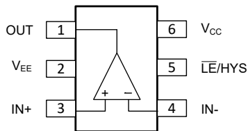
Figure 5-2. DCK Package 6-Pin SC70 Top View (Preview)
