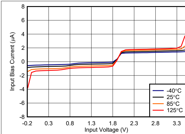
Figure 6-15. Bias Current vs. Input Voltage, 3.3 V
