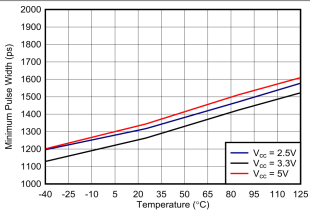
Figure 6-39. Minimum Pulse Width vs. Temperature
