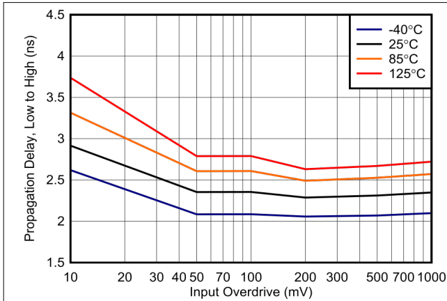
Figure 6-33. Propagation Delay, Low to High, 3.3 V
