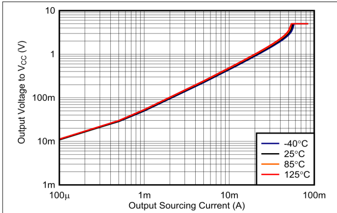
Figure 6-21. Output Voltage vs. Output Sourcing Current, 5 V
