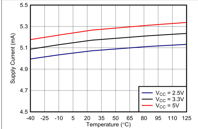
Figure 6-25. TLV3601 Supply Current vs. Temp (Output Low)
