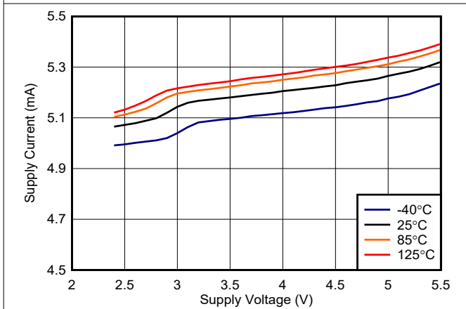
Figure 6-23. TLV3601 Supply Current vs. Voltage (Output Low)
