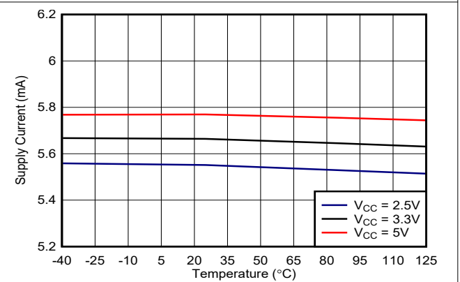
Figure 6-30. TLV3603 Supply Current vs. Temp (Output High)
