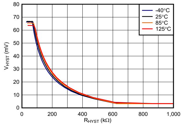
Figure 6-12. TLV3603 Hysteresis vs. Resistance, 3.3 V
