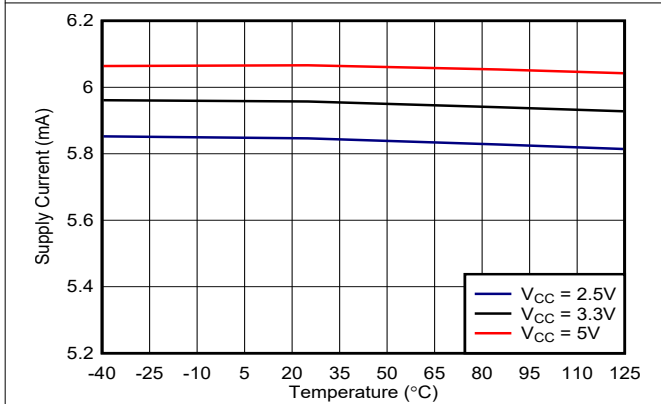
Figure 6-29. TLV3603 Supply Current vs. Temp (Output Low)
