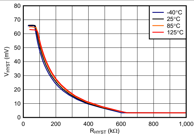
Figure 6-13. TLV3603 Hysteresis vs. Resistance, 5 V
