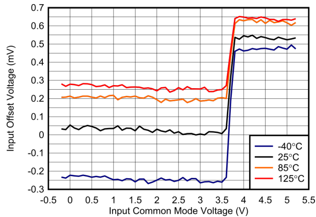
Figure 6-9. Offset Voltage vs. Common-Mode Voltage, 5 V
