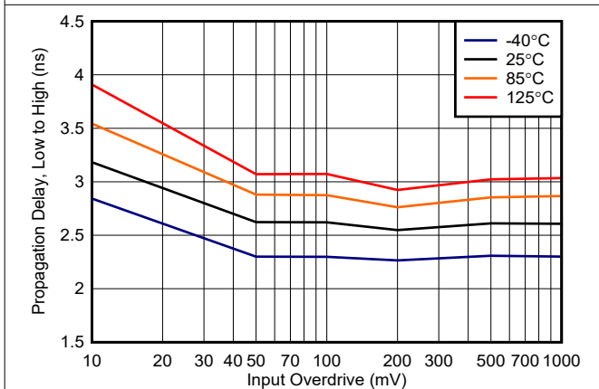
Figure 6-31. Propagation Delay, Low to High, 2.5 V
