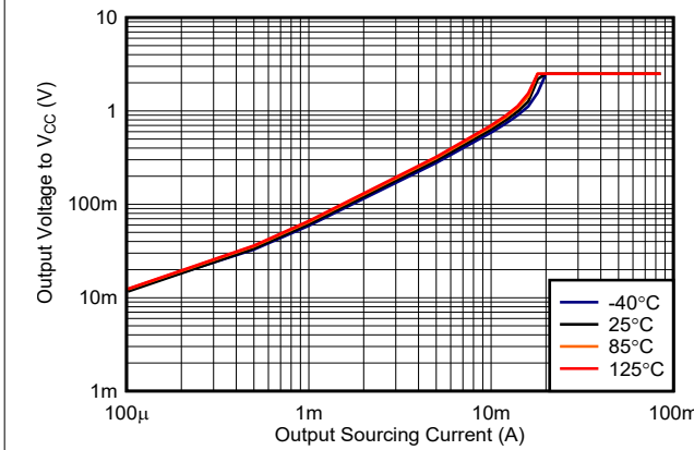
Figure 6-17. Output Voltage vs. Output Sourcing Current, 2.5 V
