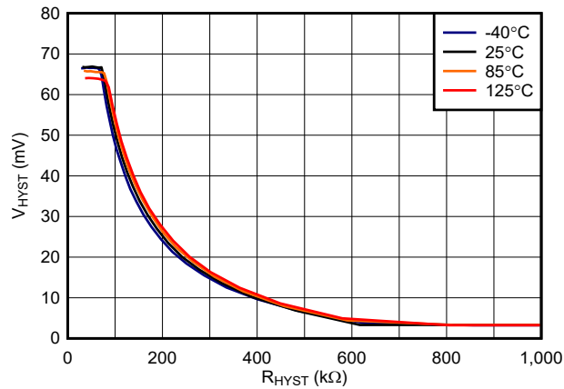
Figure 6-11. TLV3603 Hysteresis vs. Resistance, 2.5 V
