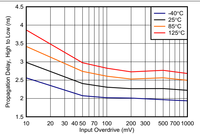
Figure 6-34. Propagation Delay, High to Low, 3.3 V
