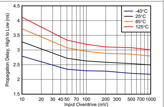
Figure 6-32. Propagation Delay, High to Low, 2.5 V
