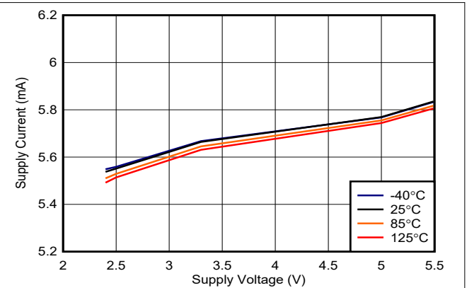
Figure 6-28. TLV3603 Supply Current vs. Voltage (Output High)
