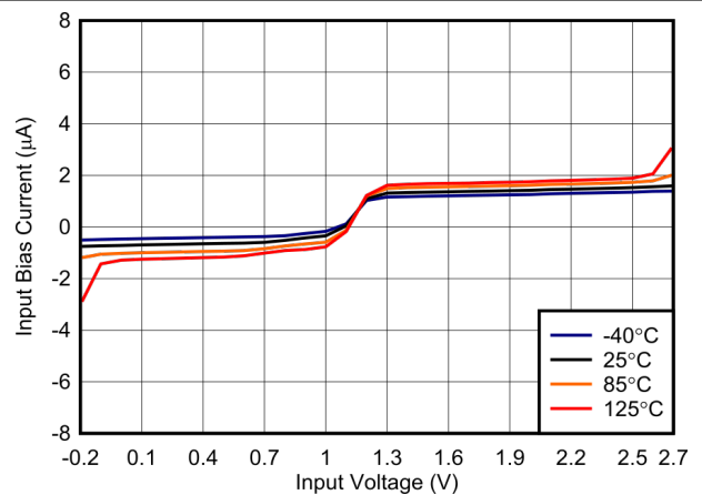
Figure 6-14. Bias Current vs. Input Voltage, 2.5 V
