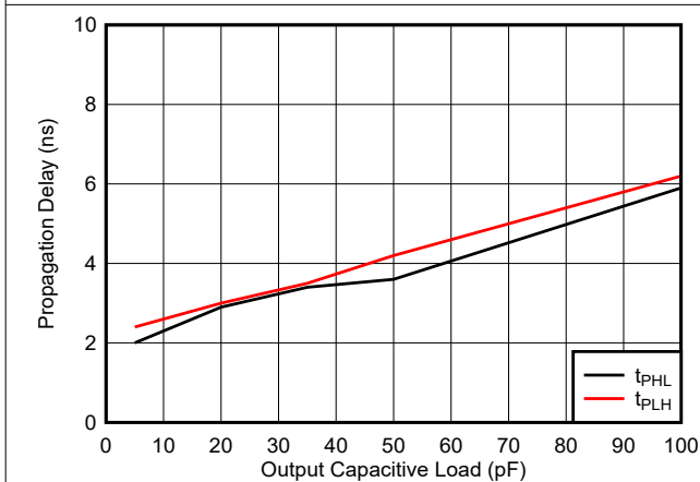
Figure 6-37. Propagation Delay vs. Load Capacitance, 3.3 V
