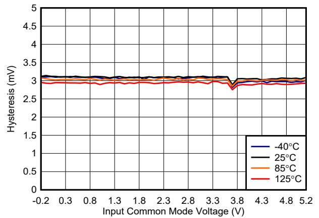
Figure 6-10. Hysteresis vs. Common-Mode Voltage, 5 V
