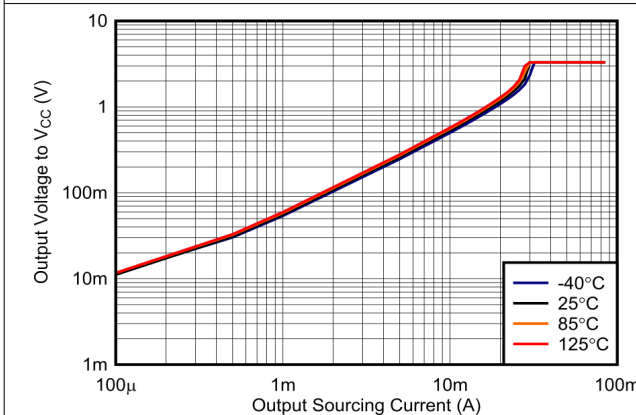
Figure 6-19. Output Voltage vs. Output Sourcing Current, 3.3 V
