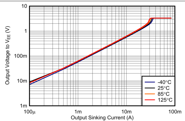
Figure 6-20. Output Voltage vs. Output Sinking Current, 3.3 V
