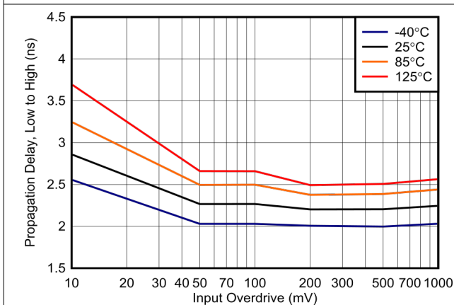
Figure 6-35. Propagation Delay, Low to High, 5 V
