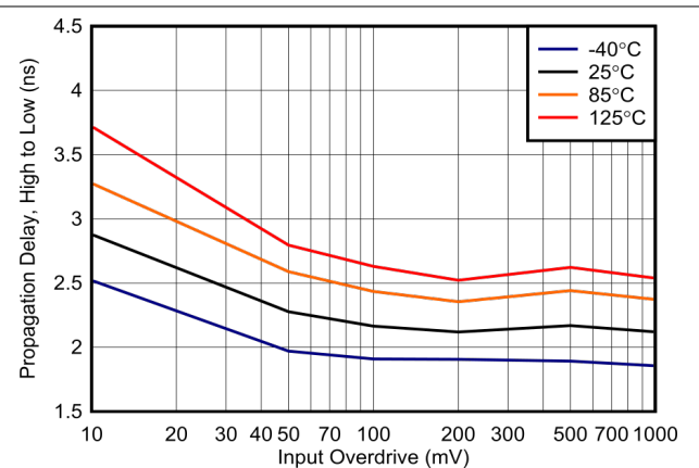
Figure 6-36. Propagation Delay, High to Low, 5 V
