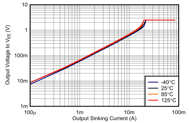
Figure 6-18. Output Voltage vs. Output Sinking Current, 2.5 V
