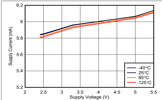
Figure 6-27. TLV3603 Supply Current vs. Voltage (Output Low)
