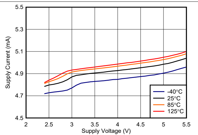
Figure 6-24. TLV3601 Supply Current vs. Voltage (Output High)
