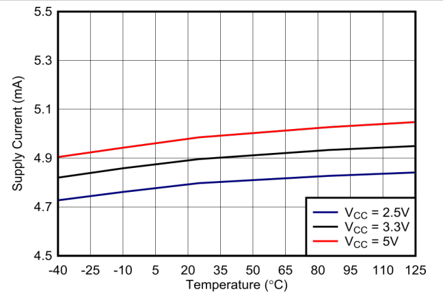
Figure 6-26. TLV3601 Supply Current vs. Temp (Output High)
