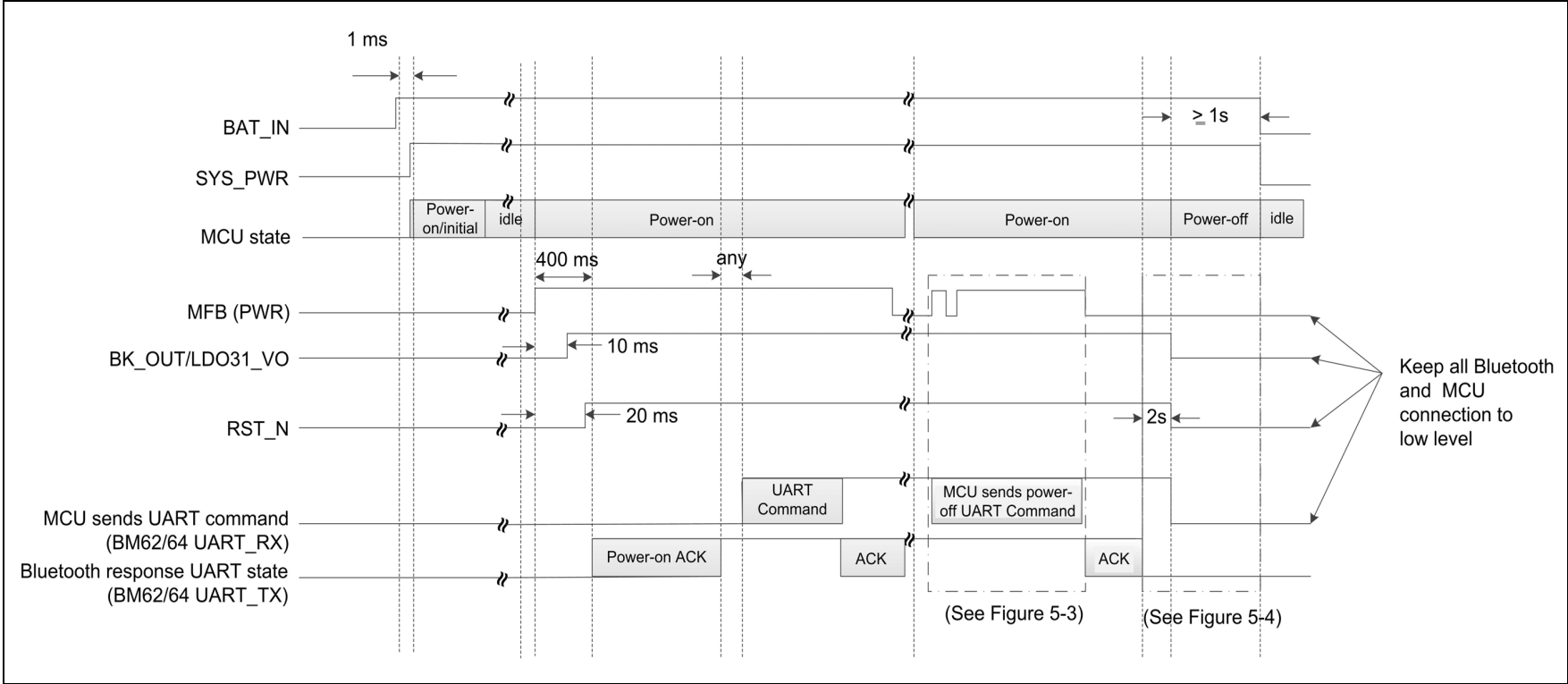
FIGURE 5-3: POWER-ON/OFF SEQUENCE
