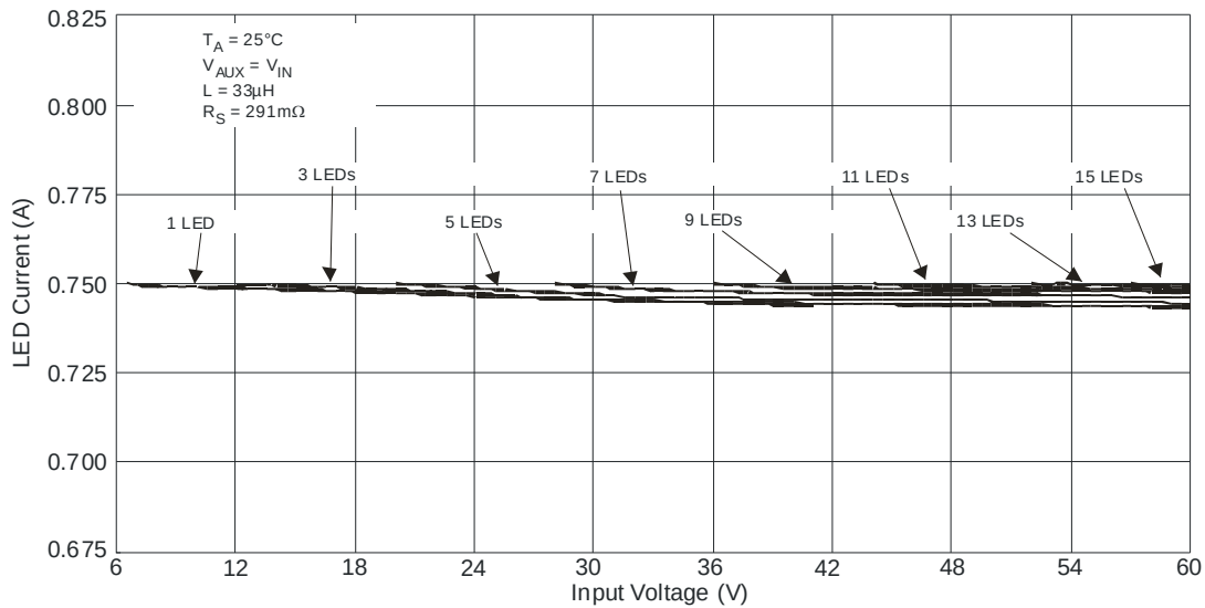
Figure 14. I_{\text{LED}} vs. Input Voltage and Number of LED
