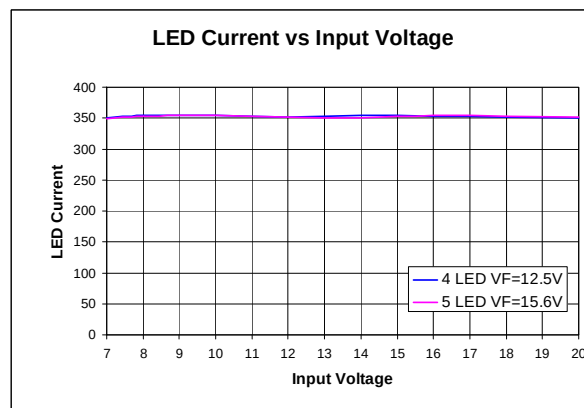
Figure 60. Line regulation
