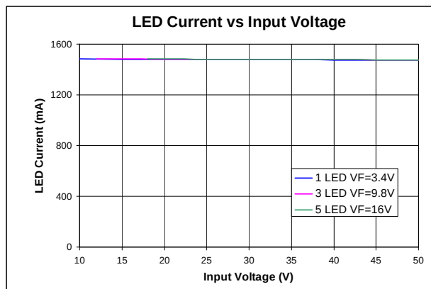
Figure 54. Line regulation
