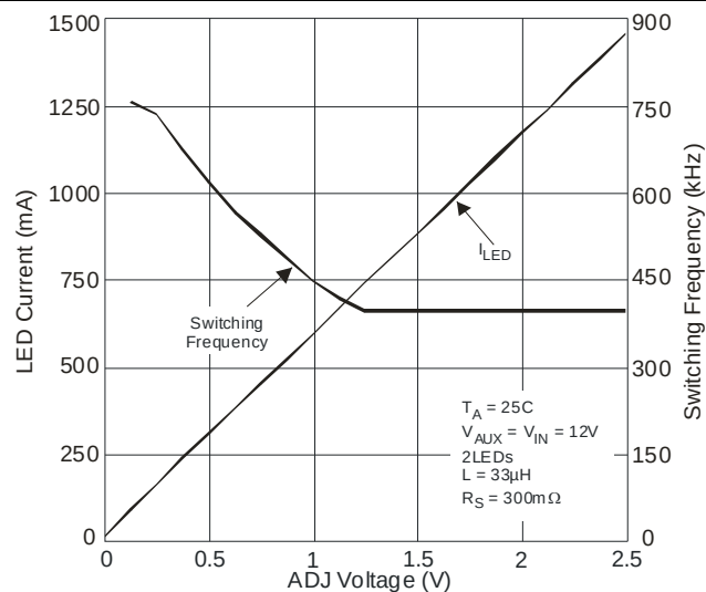
Figure 2. Buck LED Current, Switching Frequency vs. V_{ADJ}
