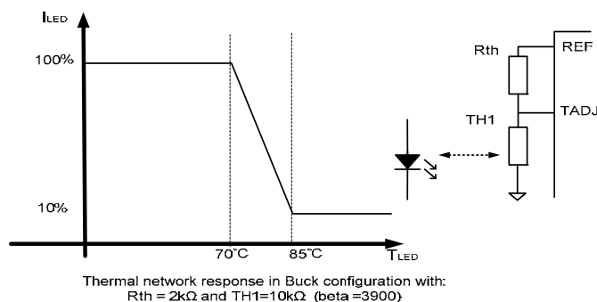
Figure 47. Thermal feedback network
