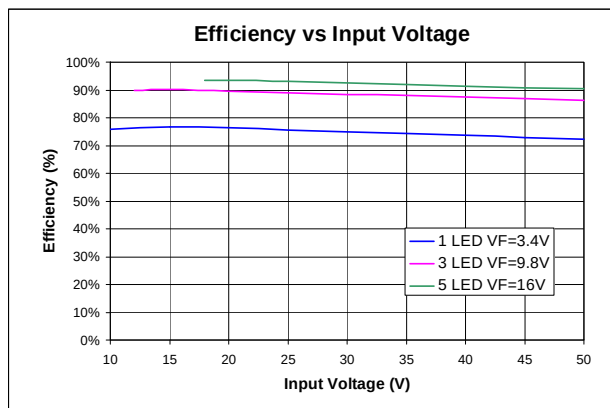
Figure 53. Efficiency
