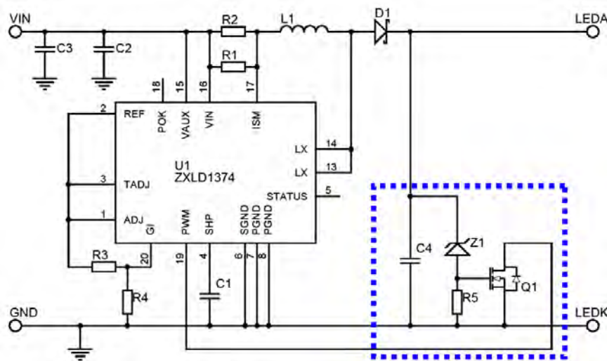
Figure 50. OVP Circuit
