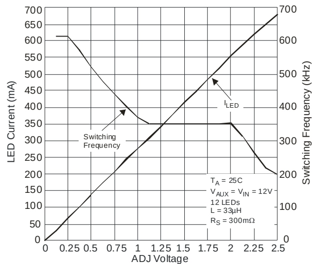
Figure 4. Boost LED Current, Switching Frequency vs. V_{ADJ}
