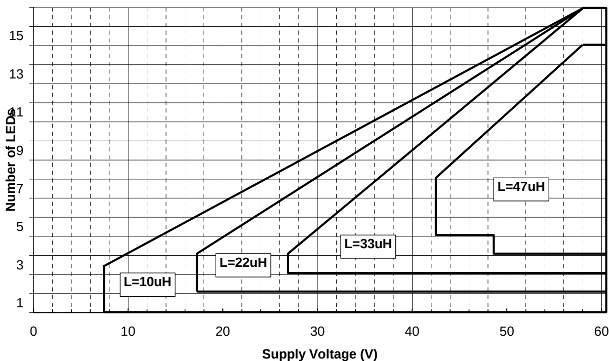
Figure 35: 750mA Buck mode inductor selection for target frequency > 500kHz
