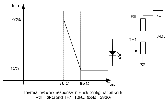
Curve showing LED current vs. T_{LED}
