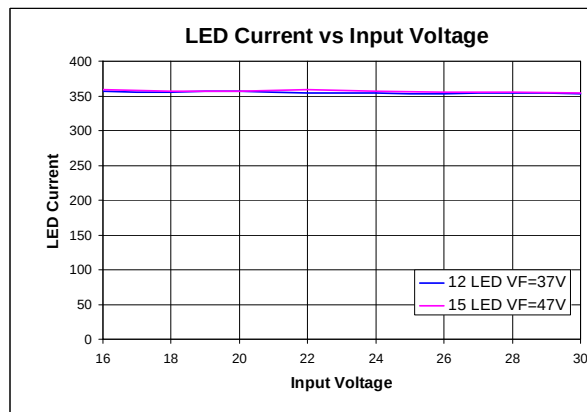
Figure 57. Line regulation
