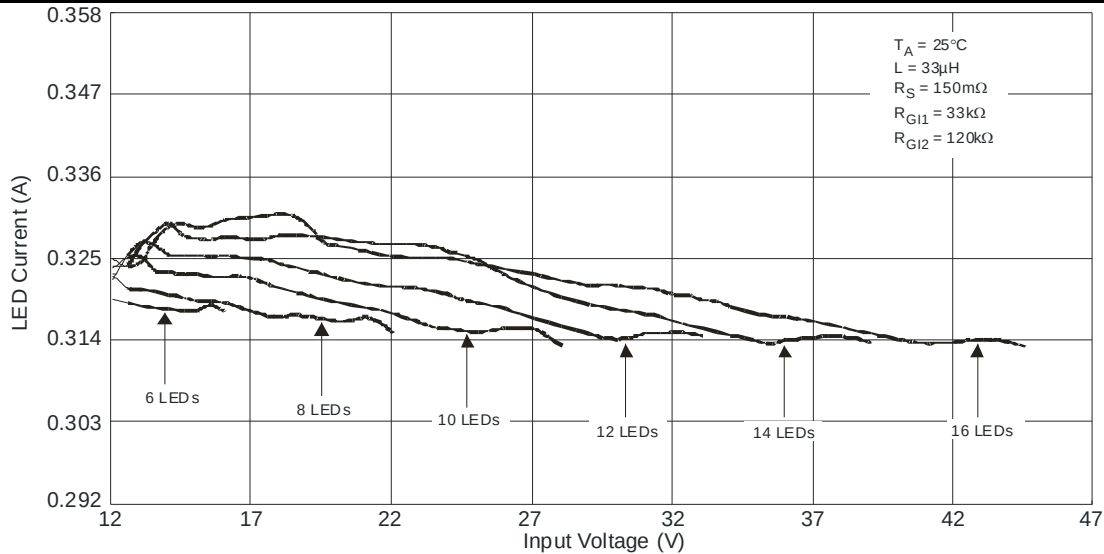
Figure 17. I_{\text{LED}} vs. Input and Number of LED
