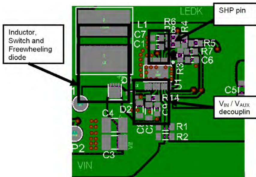
Figure 51. Circuit Layout
