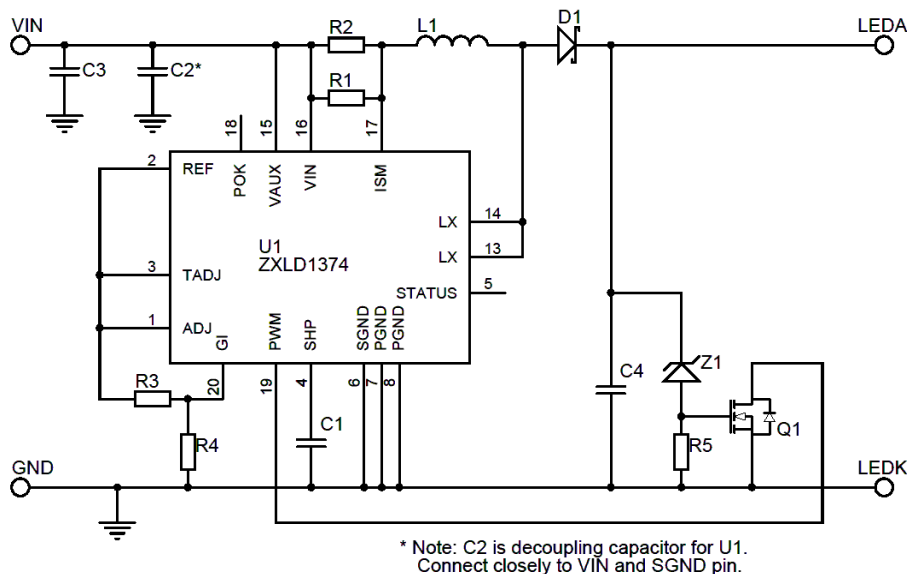
Figure 55. Application circuit of 350mA Boost LED driver
