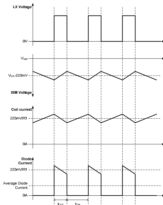
Figure 29. Operating Waveforms (Boost and Buck-boost Modes)
