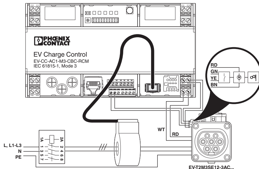
Connection diagram
