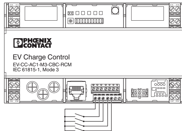
Connection diagram
