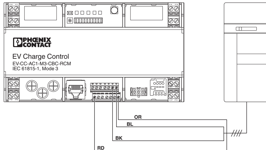
Connection diagram
