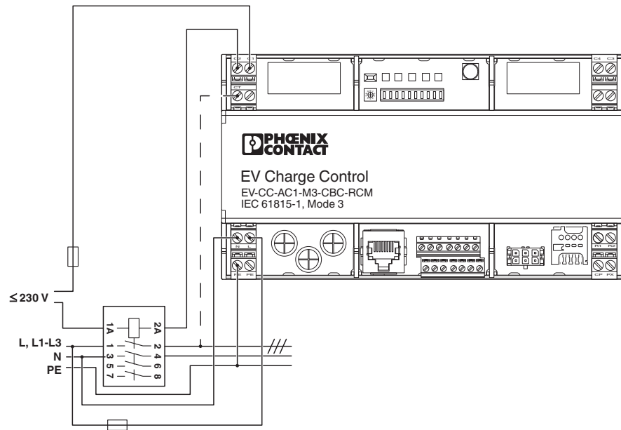
Connection diagram
