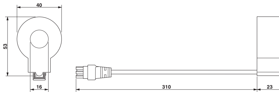
Dimensional drawing
