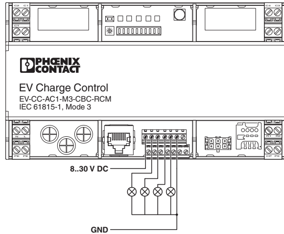
Connection diagram
