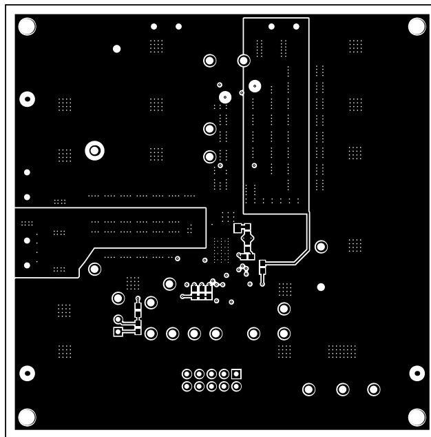
Figure 68. EVM Bottom Layer
