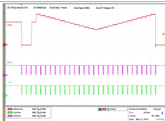
Figure 19. 17 Sequenced Events – I2C Write/Read with PEC
