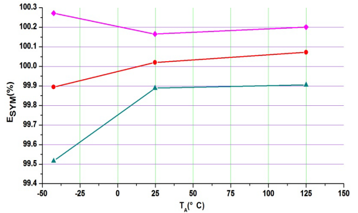
Total Output Error versus Ambient Temperature
