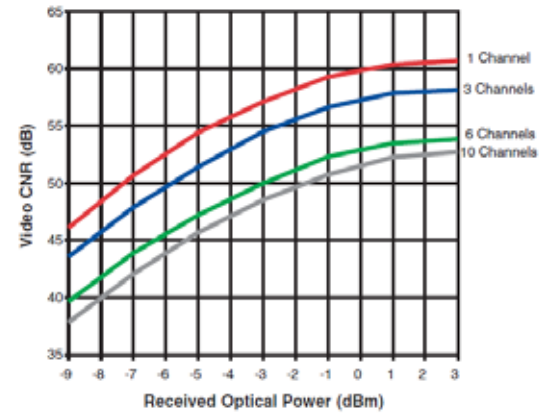
Carrier-to-Noise Performance:
