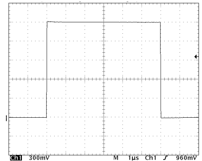
Typical Output Waveform, 1500V (1μs/Div horizontal scale, 300V/Div vertical scale)
