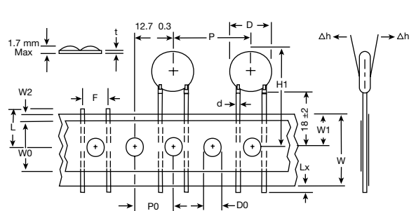
Straight Lead T36 (Ammo Box) and T19 (Reel) (7.5mm Lead Spacing)
