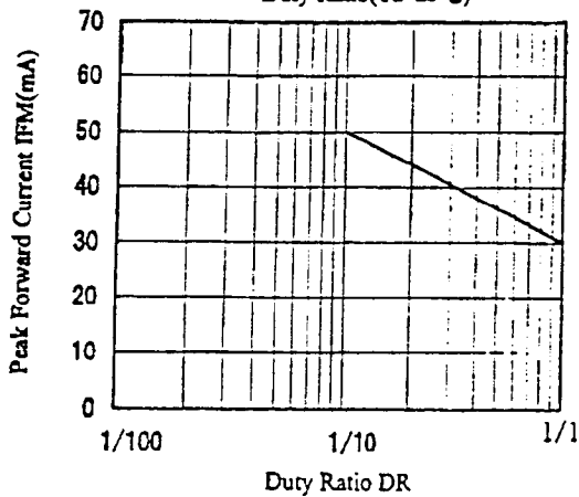
Peak Forward Current vs. Duty Ratio ( T_a=25^\circ\text{C} )
