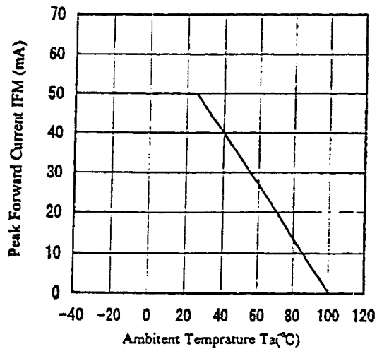
Peak Forward Current Derating Curve
