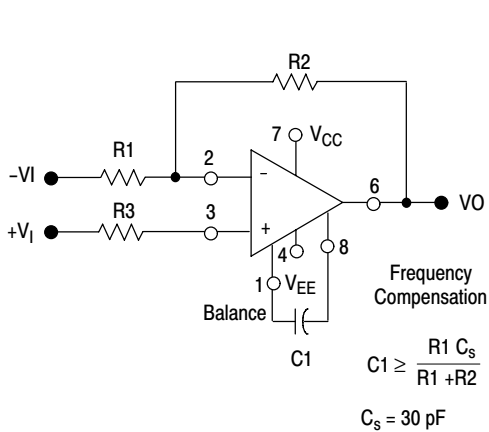
Figure 14. Single-Pole Compensation
