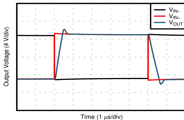
Figure 7-43. Settling Time
