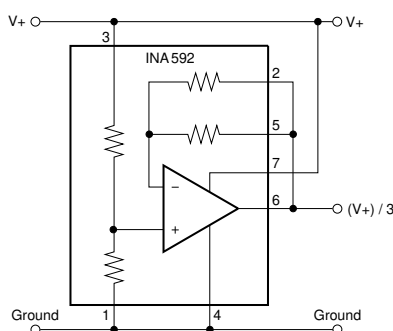
Figure 9-7. Pseudoground Generator
