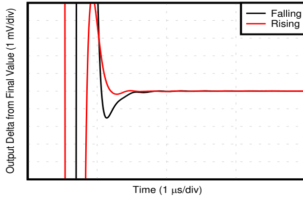
Figure 7-43. Settling Time
