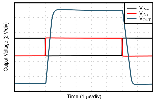
Figure 7-44. Settling Time
