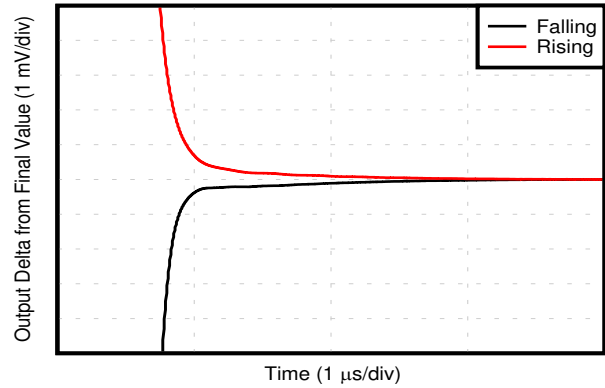
Figure 7-44. Settling Time
