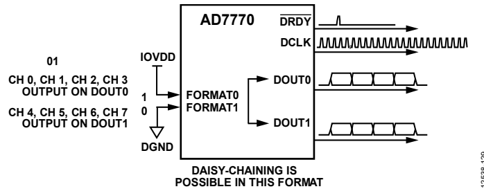
Figure 114. FORMATx Pin Configuration—FORMAT0 = 1, FORMAT1 = 0
