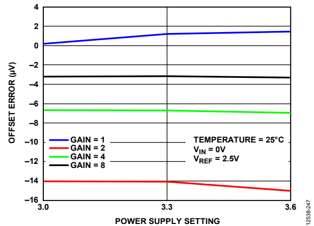
Figure 47. Offset Error vs. Power Supply Setting, Low Power Mode
