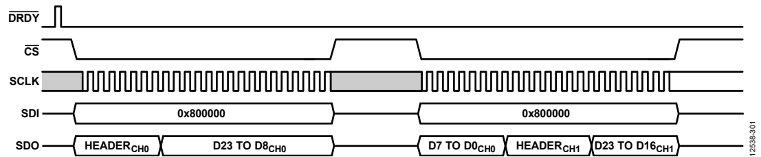
Figure 105. SPI Used to Read Back the \Sigma - \Delta ADC Data, in 24-Bit Frames
