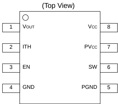
Fig.2 BD9102FVM BD9104FVM
