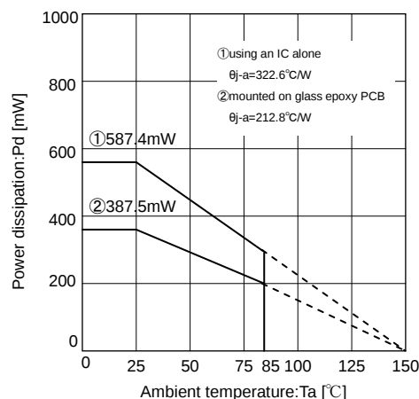
Fig.50 Thermal derating curves
