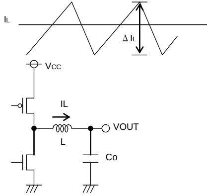
Fig.51 Output ripple current
