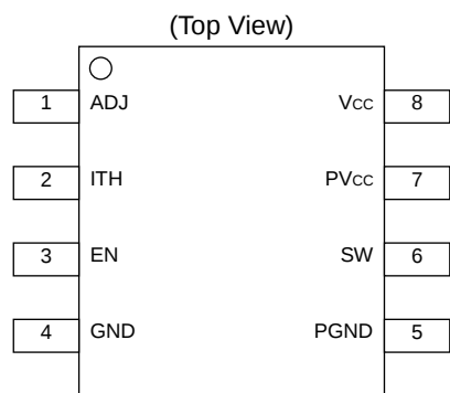
Fig.3 BD9106FVM
