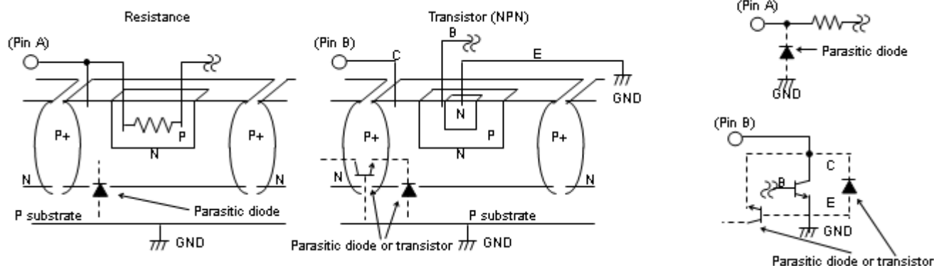
Fig.60 Simplified structure of monorisc IC
