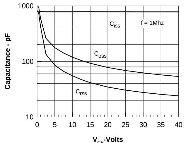
Figure 6. Capacitance Curves
