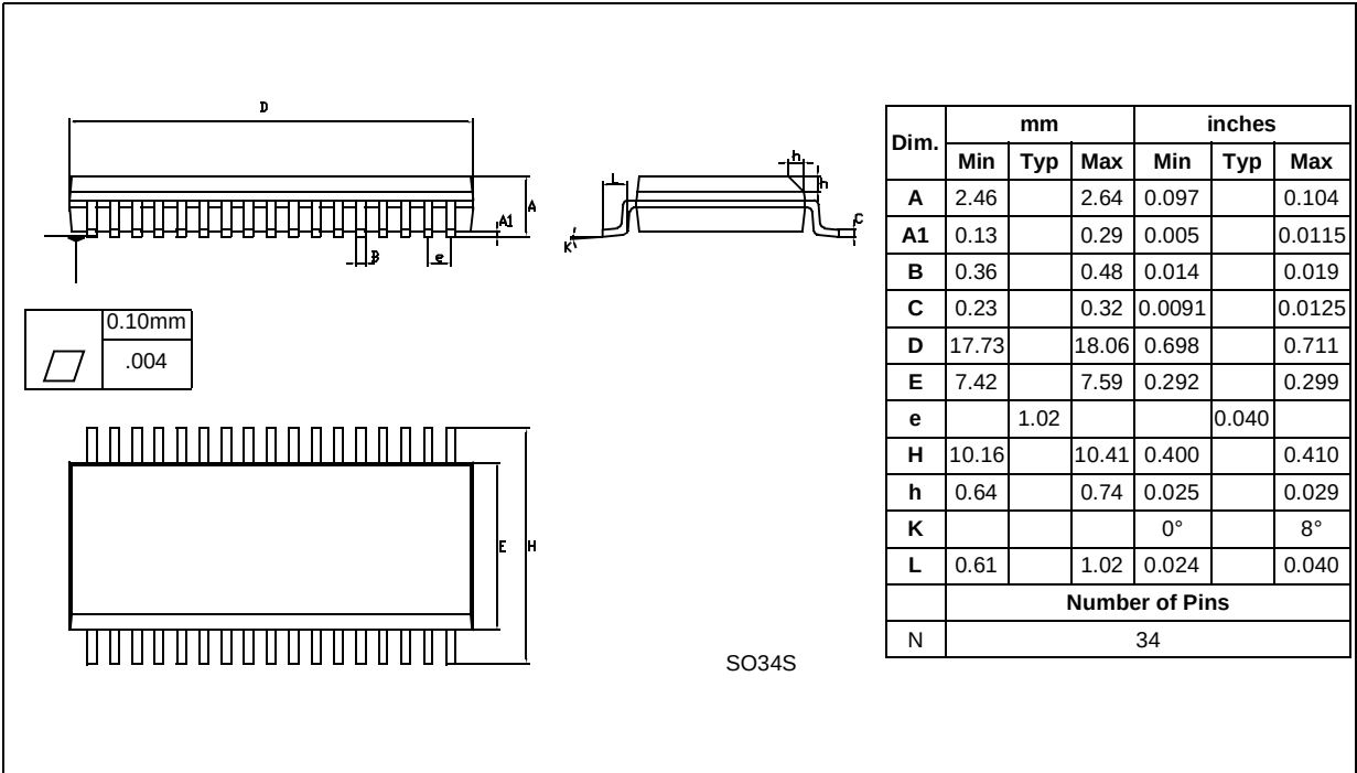
Figure 93. 34-Pin Plastic Small Outline Package
