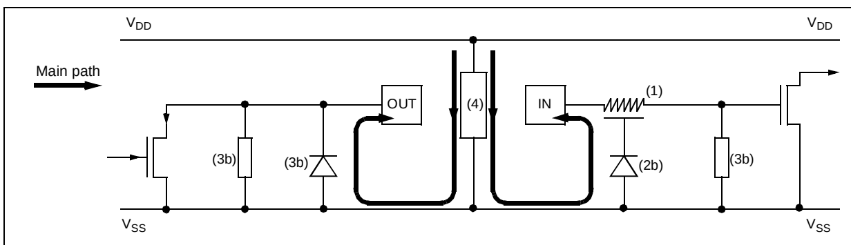
Figure 67. Multisupply Configuration
