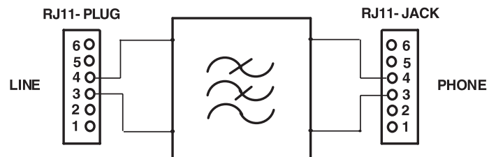
Z-321NF-50 Block Schematic
