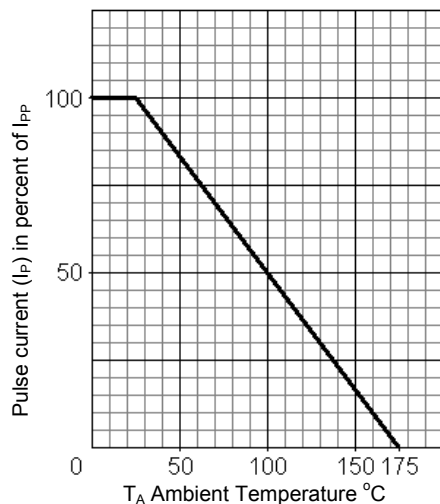
FIG. 4 Derating Curve
