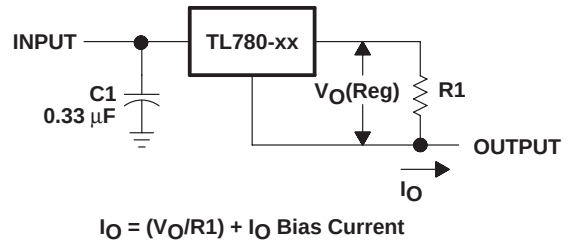
Figure 3. Current Regulator
