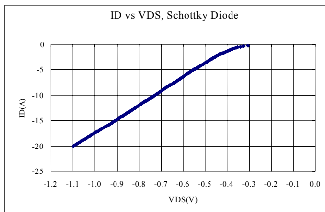
Figure 9 – Diode Voltage vs Current
