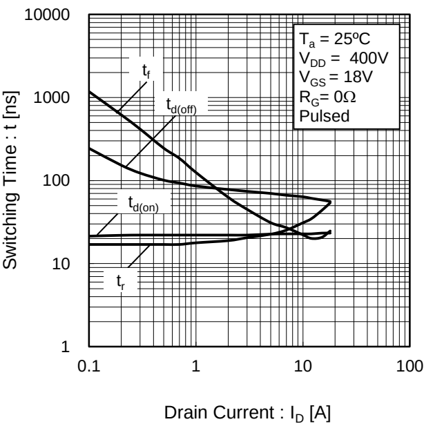
Fig.14 Switching Characteristics
