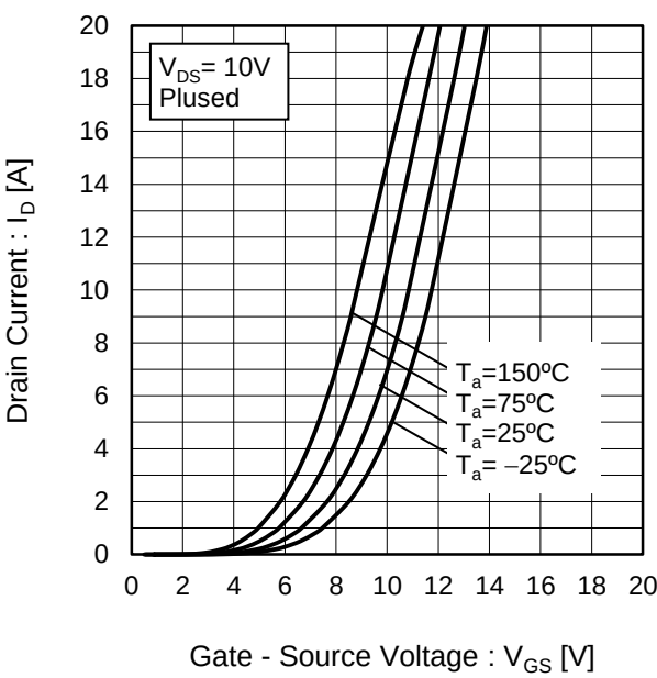
Fig.6 Typical Transfer Characteristics (II)
