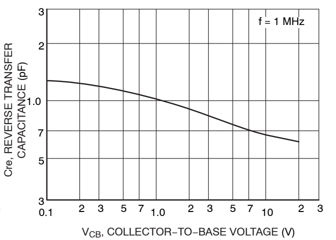
Figure 6. C_{re} - V_{CB}
