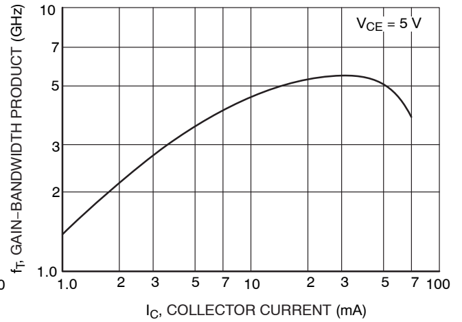
Figure 4. f_T - I_C
