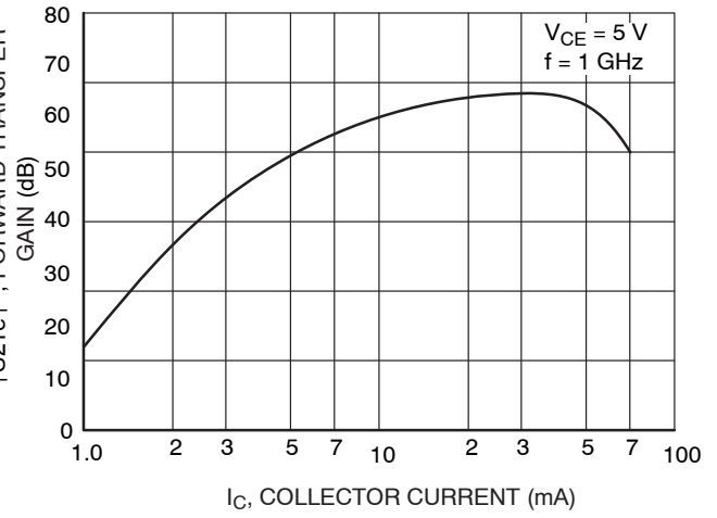
Figure 8. |S_{21e}|^2 - I_C
