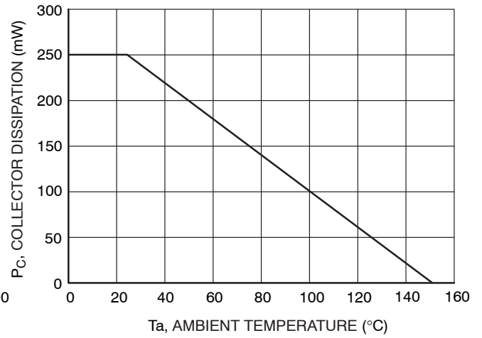
Figure 10. P_C - T_a
