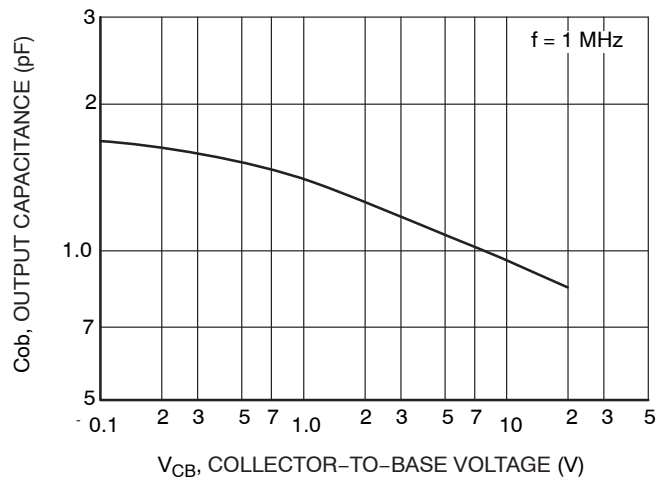
Figure 5. C_{ob} - V_{CB}
