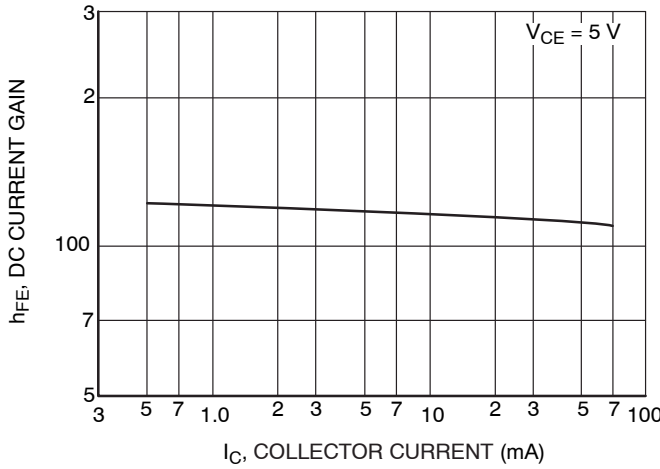
Figure 3. h_{FE} - I_C
