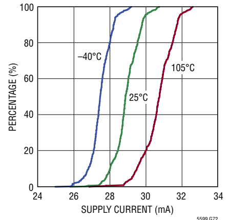
Supply Current Cumulative Distribution
