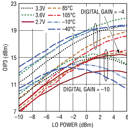
Output IP3 vs LO Power at f_{LO} = 900MHz
