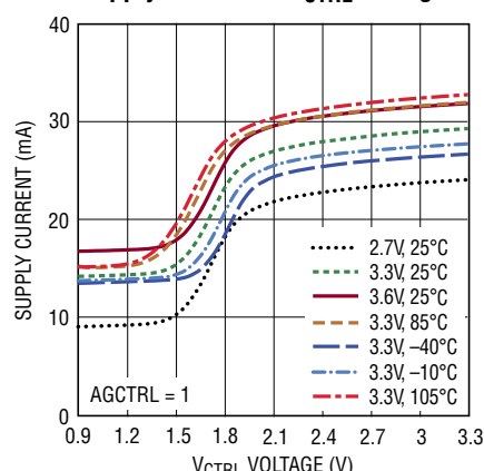
Supply Current vs V_{CTRL} Voltage
