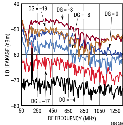
LO Leakage vs LO Frequency and Digital Gain Setting After Calibration at DG = -4
