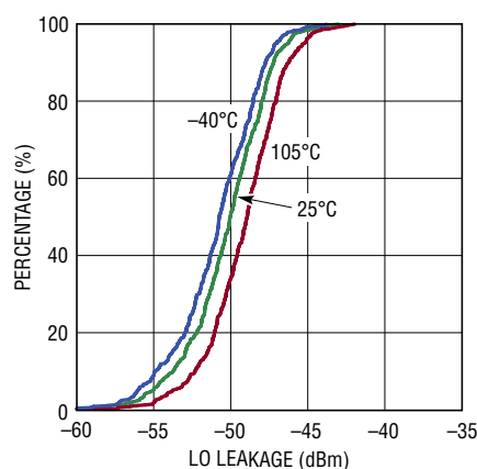
LO Leakage Cumulative Distribution
