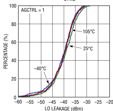
LO Leakage Cumulative Distribution for V_{CTRL} = 1.75V
