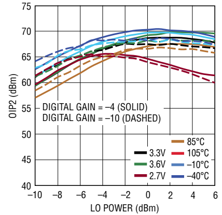
Output IP2 vs LO Power at f_{LO} = 150MHz
