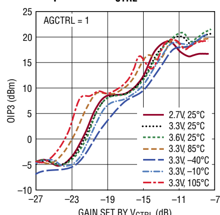
Output IP3 vs V_{CTRL} Gain
