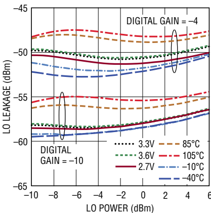
LO Leakage vs LO Power at f_{LO} = 150MHz
