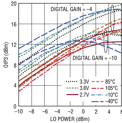
Output IP3 vs LO Power at f_{LO} = 1260MHz
