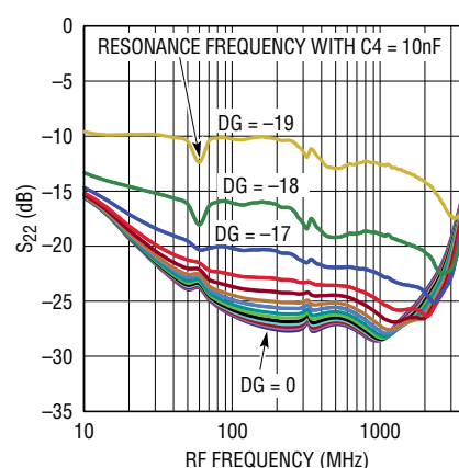
RF Return Loss
