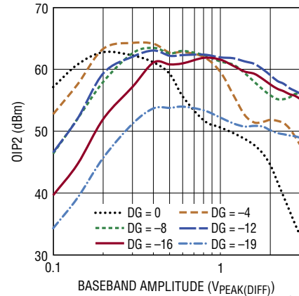
Output IP2 vs Baseband Amplitude
