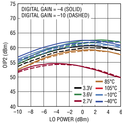
Output IP2 vs LO Power at f_{LO} = 500MHz
