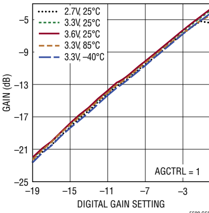
Gain vs Digital Gain Setting
