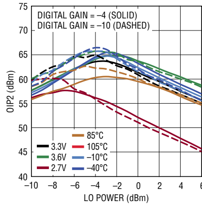
Output IP2 vs LO Power at f_{LO} = 900MHz
