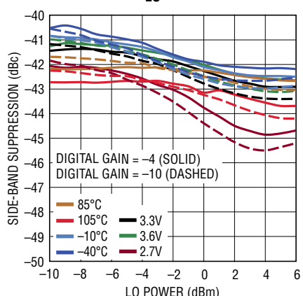
Side-Band Suppression vs LO Power at f_{LO} = 1260MHz
