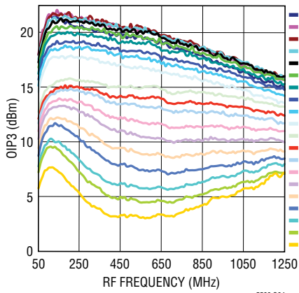
Output IP3 vs RF Frequency and Digital Gain Setting
