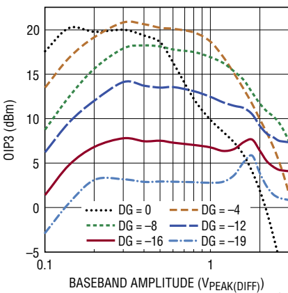
Output IP3 vs Baseband Amplitude
