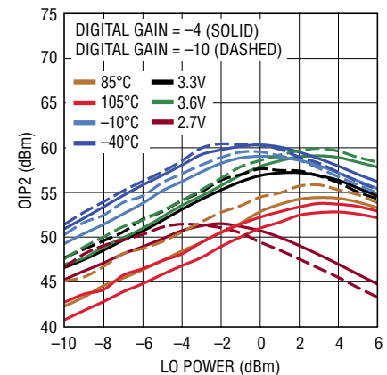
Output IP2 vs LO Power at f_{LO} = 1260MHz
