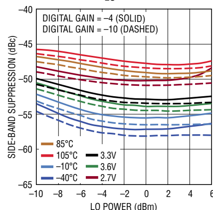
Side-Band Suppression vs LO Power at f_{LO} = 500MHz
