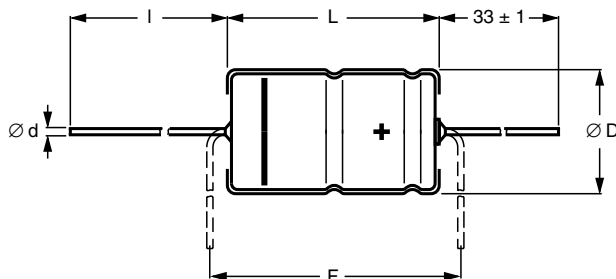
Fig.4 Form AA
