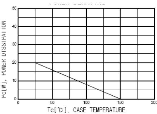
Fig 3. Power derating
