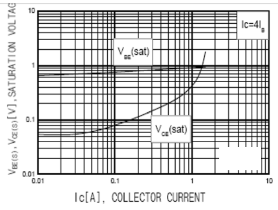
Fig 4. Saturation Voltage
