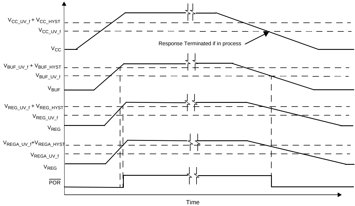
Figure 6. Powerup Timing
