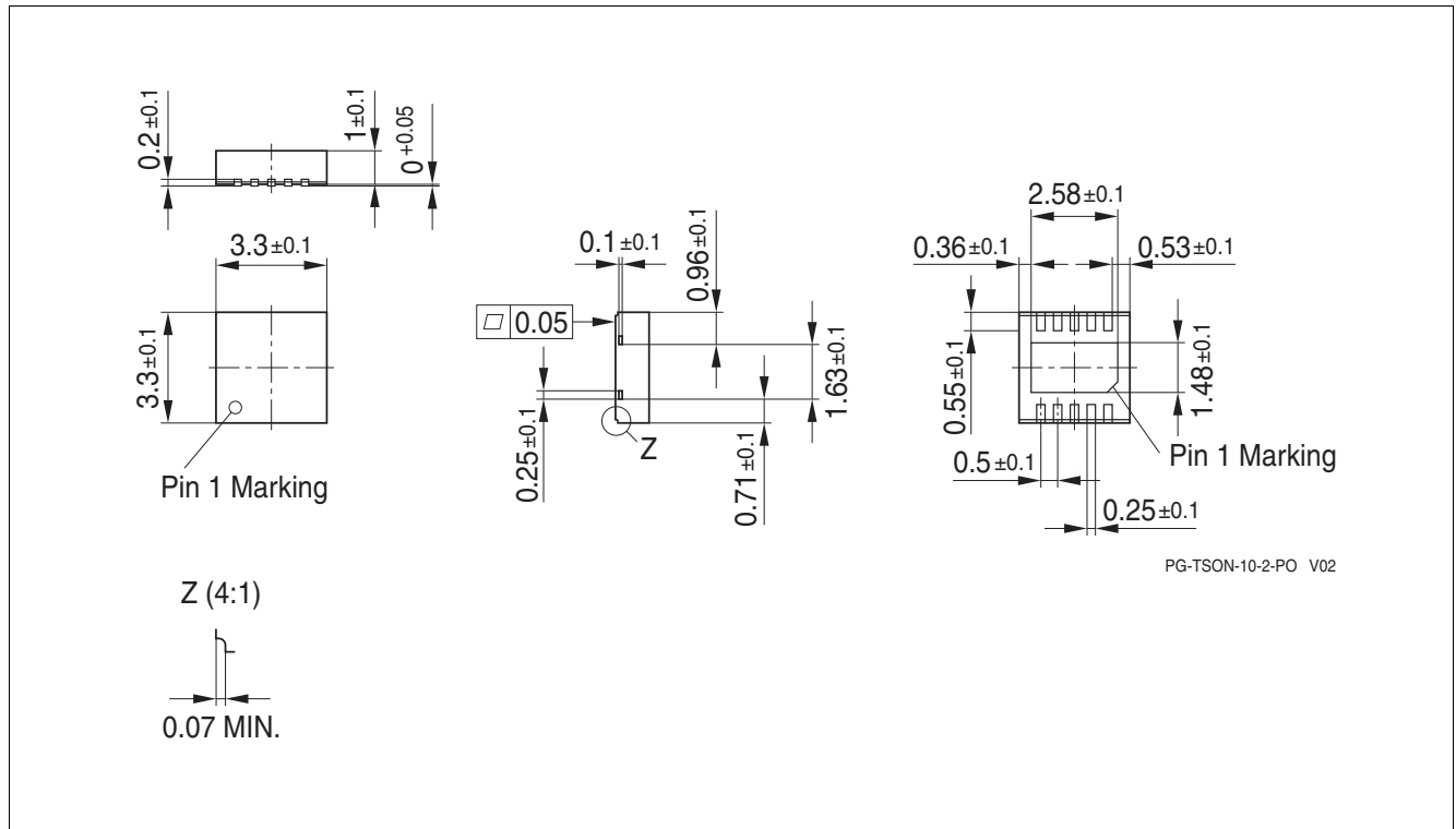
Figure 8 PG-TSON-10
