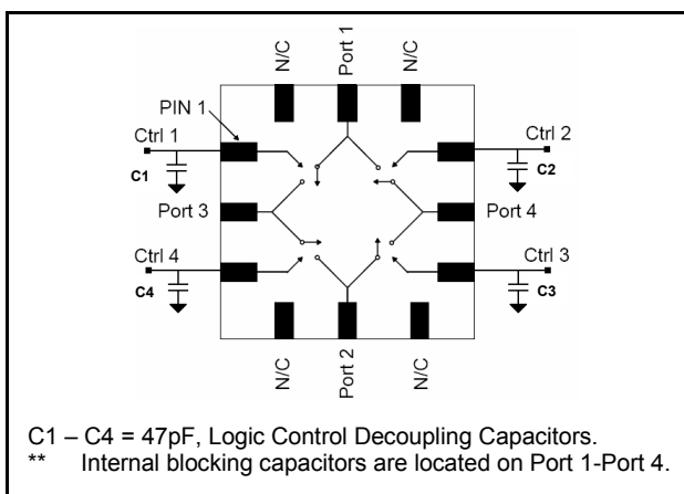
Circuit Block Diagram**
