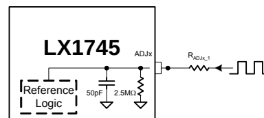
Figure 4 – LCD Bias Adjustment Input
