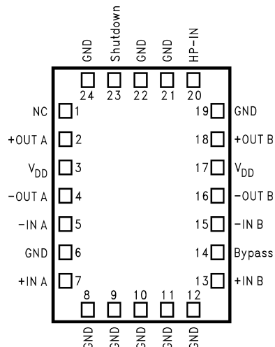
Figure 4. 24-Pin Exposed-DAP WQFN - Top View See Package Number NHW0024A
