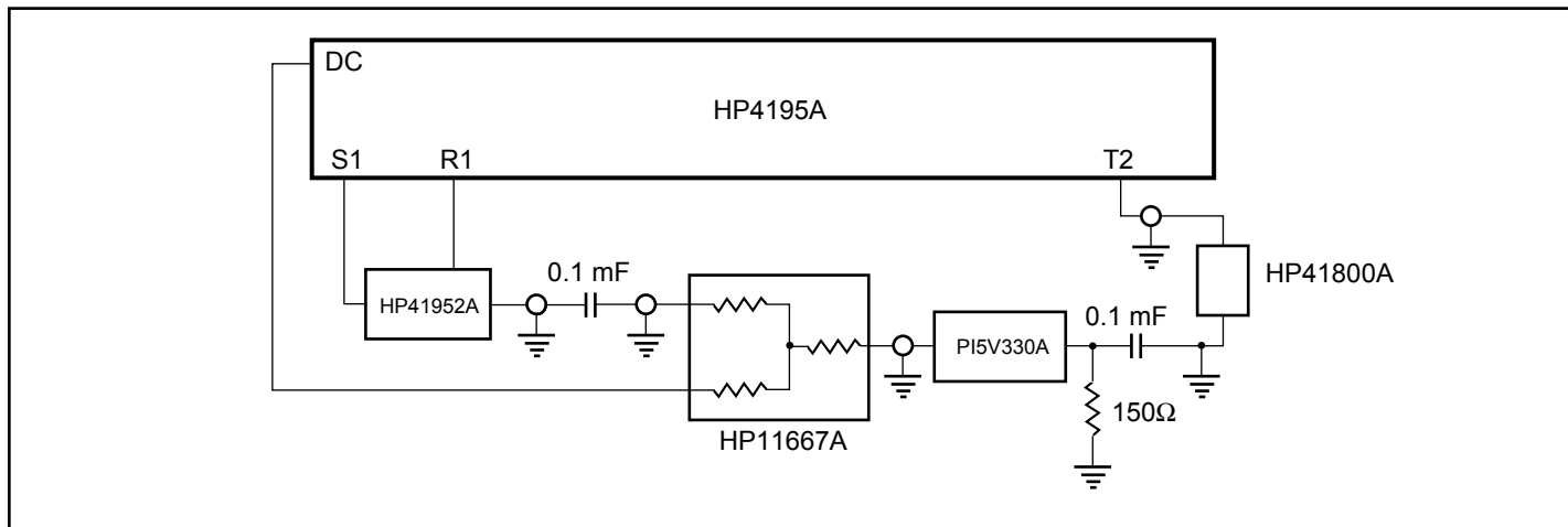
Figure 5. Differential Gain/Phase
