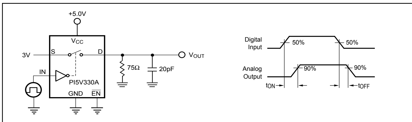
Figure 6. Switching Time
